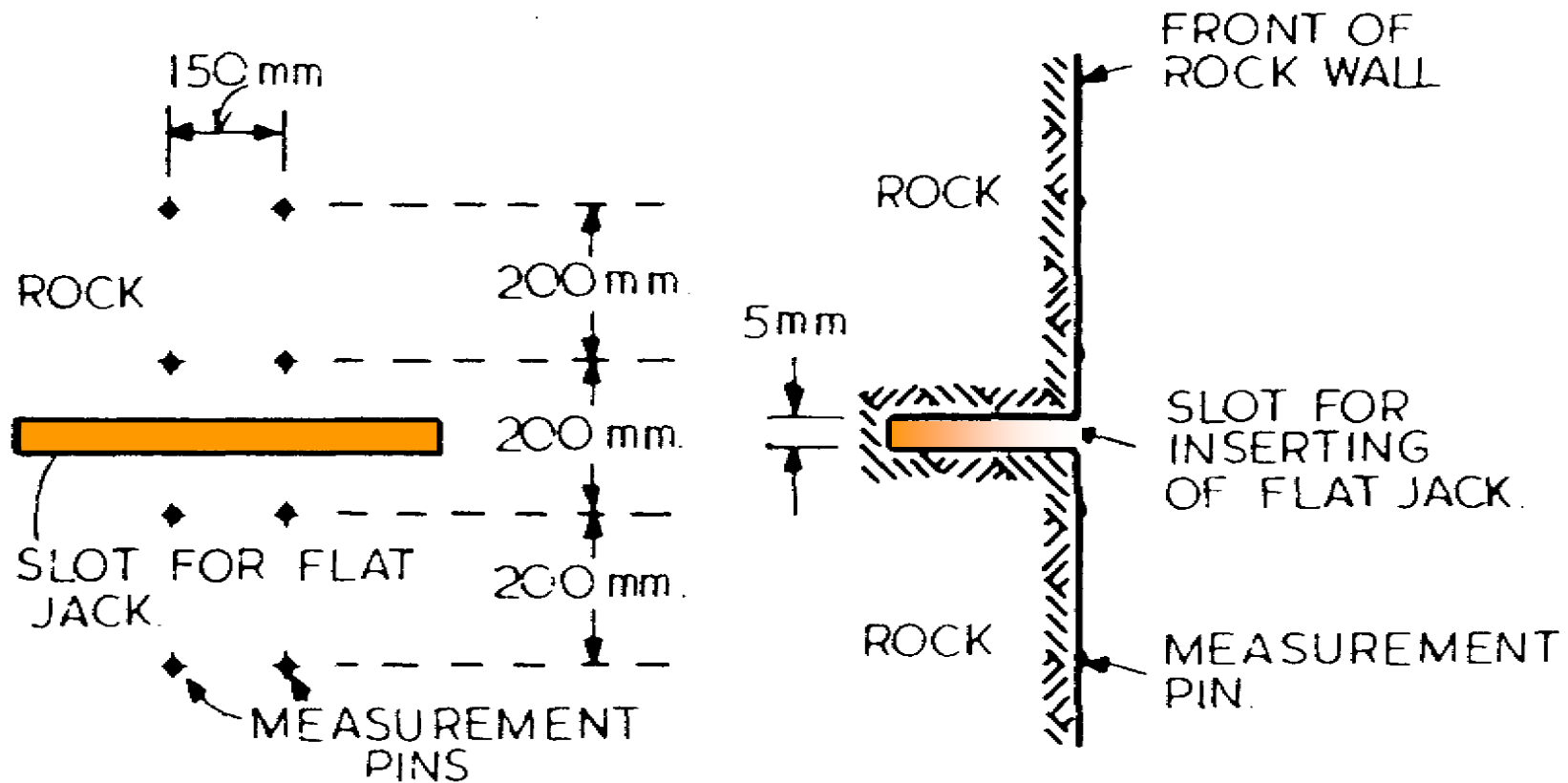
a FRONT VIEW OF SLOT IN ROCK.
