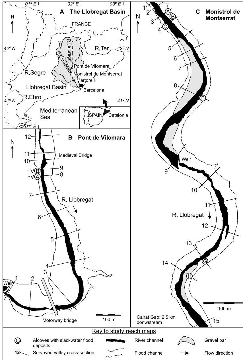
Fig. 1. Location of the Llobregat Basin in NE Spain (A). The Pont de Vilomara (B) and Monistrol de Montserrat (C) study reaches, illustrating the location of rock alcoves preserving slackwater flood deposits (sites A–H) and surveyed cross sections (numbered).
