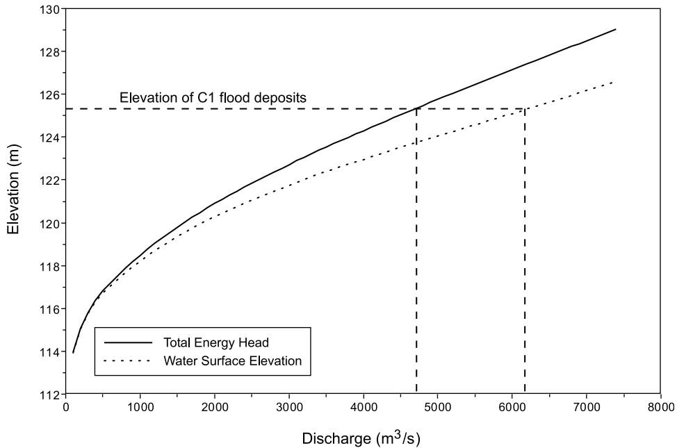
Fig. 7. Rating curve for the C1 flood deposits, dated to cal. AD 1516–1642, at cross section 3 of the Monistrol reach illustrating the discharge estimates calculated from the water surface elevations and the total energy head. The conservative discharge associated with the total energy head was considered more accurate as the palaeoflood sediments indicated a low flow velocity (close to zero) at the canyon side, therefore the water surface elevation would be higher than in the central flood channel where flow velocity was over 6 \text{ ms}^{-1} .
