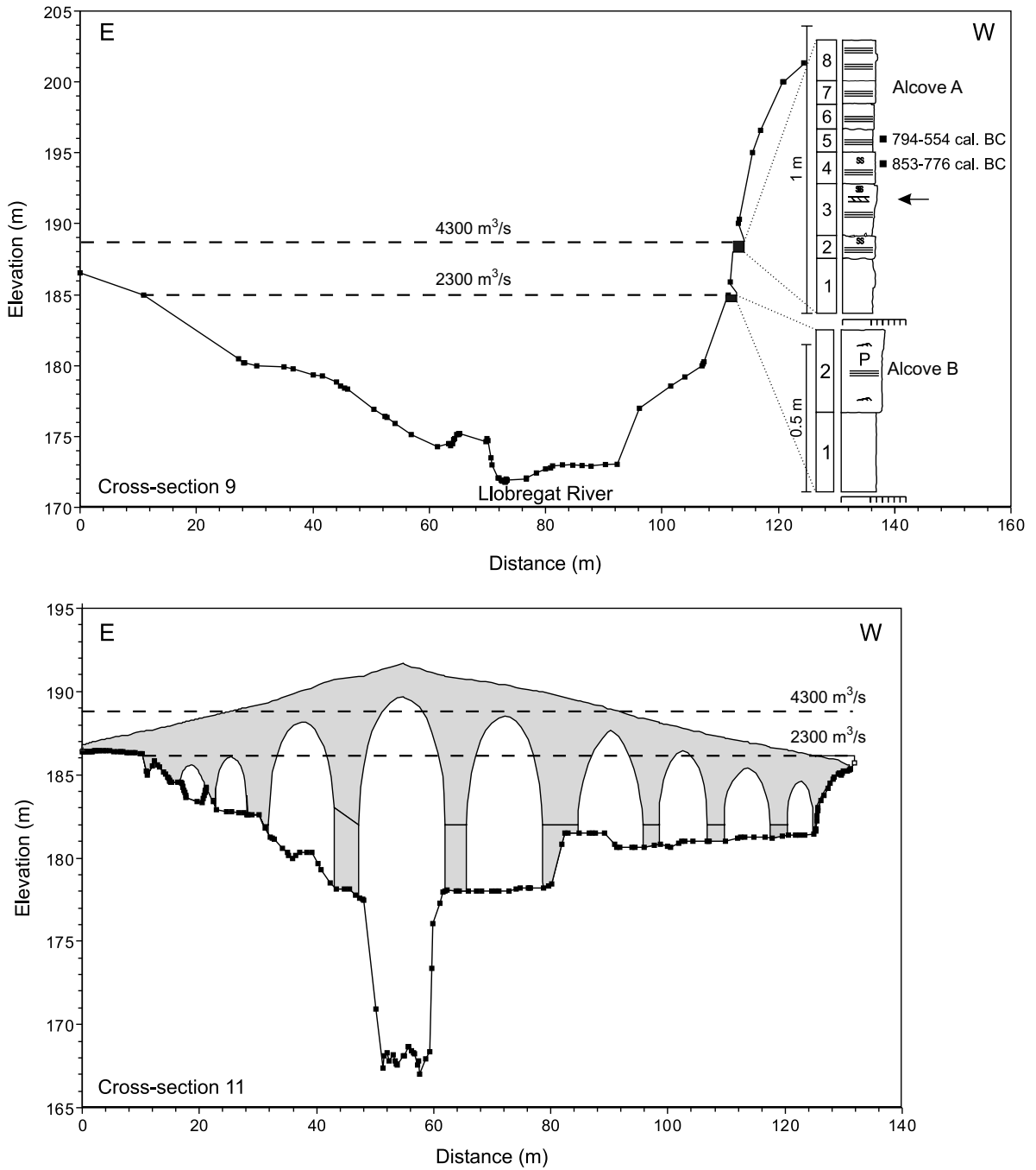
Fig. 5. Cross-section 9 of the Pont de Vilomara study reach illustrating the relative elevations of Alcoves A and B. The stratigraphy of the sedimentary profiles is also shown (refer to key in Fig. 3). Note that at this site, Alcove A preserves a record of 8 extreme flood events with two flood units dated to the Late Bronze Age. The minimum discharge estimates associated with the upper flood units are also shown. Below: the water surface elevations related to the minimum discharge estimates of the 1971 flood and flood unit A8 are plotted at cross-section 11 at the Medieval bridge. A photograph of the 1971 flood passing under the bridge enabled calibration of the hydraulic model at this reach.
