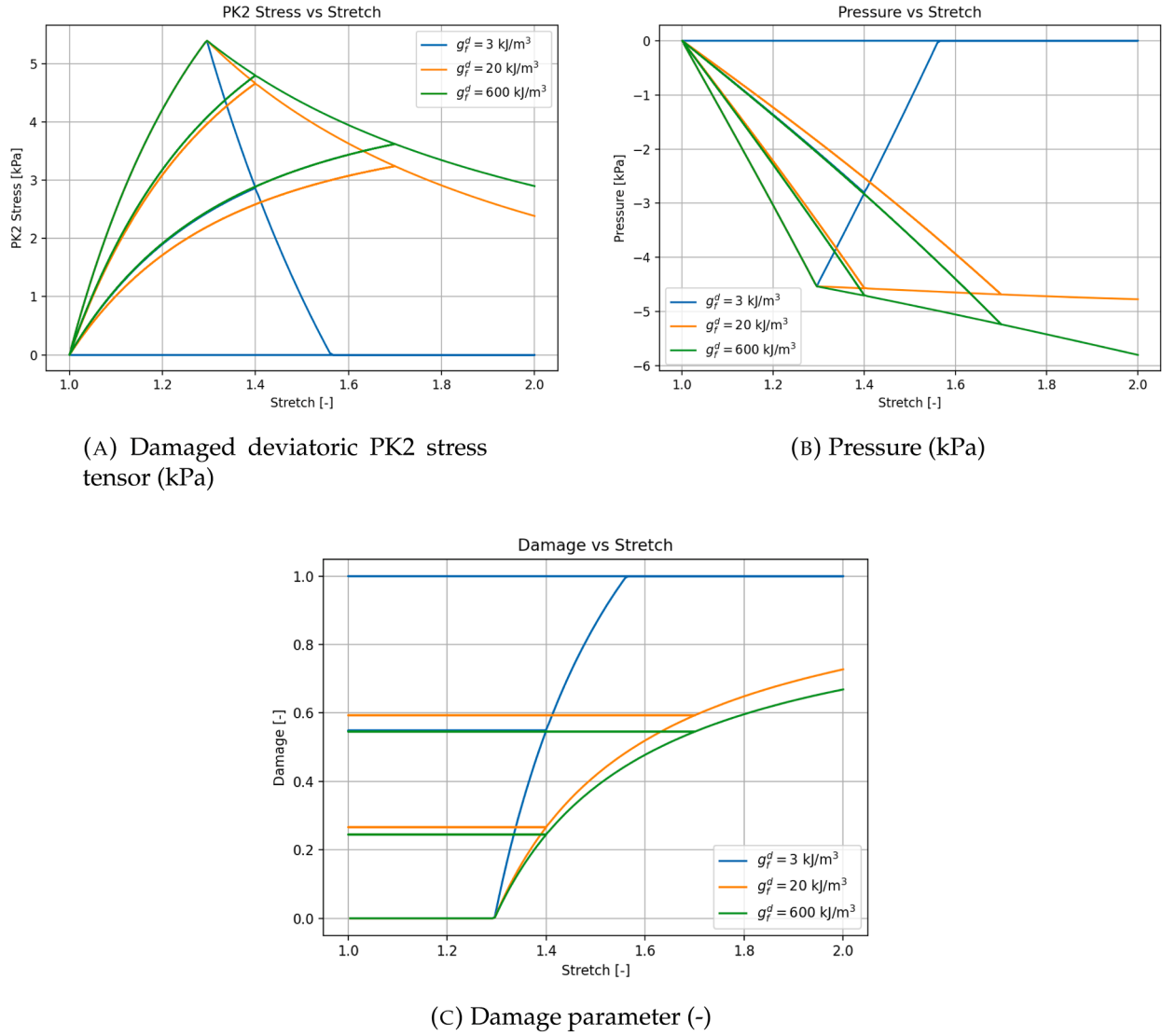
Fig. 5. Homogeneous uniaxial tension. Influence of different fracture energy per unit volume values under stretching.
