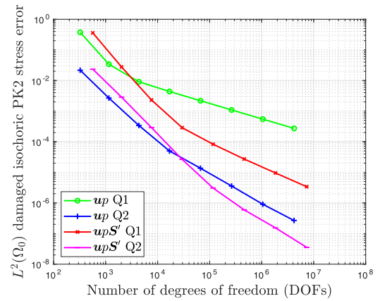
(F) Damaged isochoric PK2 stress error upon DOFs
