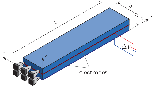
FIGURE 12 | Electrically induced bending plate. Geometry.
