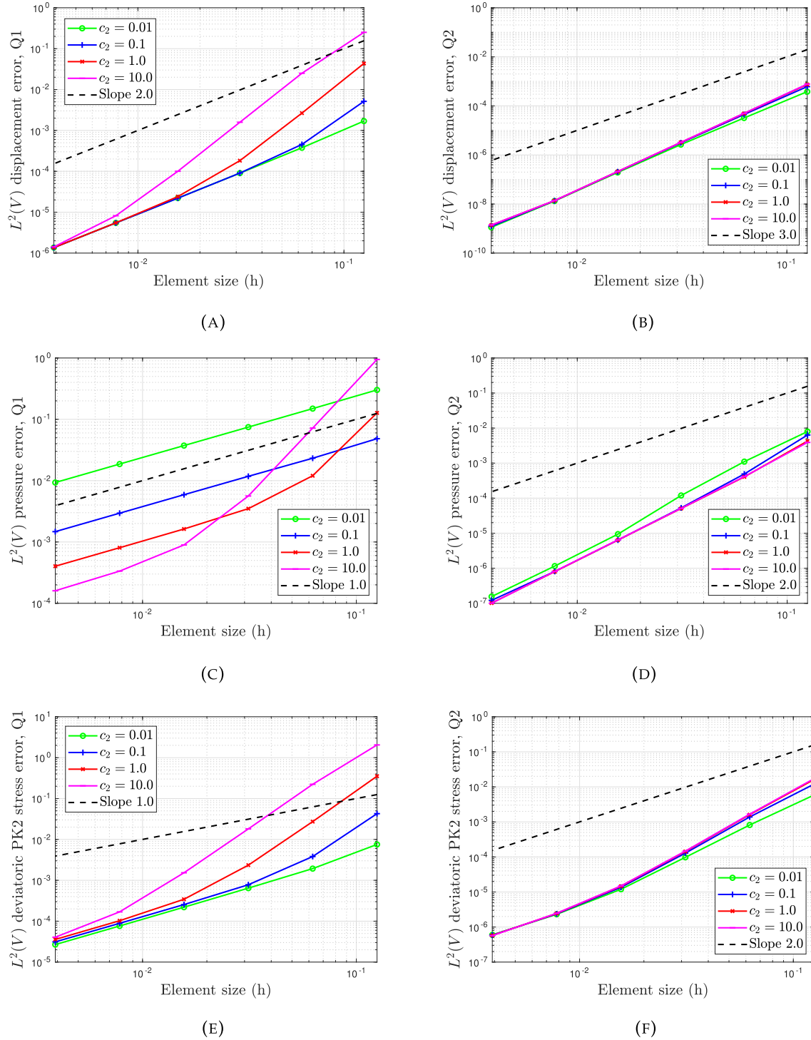
FIGURE 4 | Manufactured convergence test. Convergence rate for upS'\phi formulation upon mesh refinement. Study to determine the optimal parameter c_2 . (a) Displacement error upon mesh refinement, Q1 elements, (b) Displacement error upon mesh refinement, Q2 elements, (c) Pressure error upon mesh refinement, Q1 elements, (d) Pressure error upon mesh refinement, Q2 elements, (e) Deviatoric PK2 mechanical stress error upon mesh refinement, Q1 elements, and (f) Deviatoric PK2 mechanical stress error upon mesh refinement, Q2 elements.
