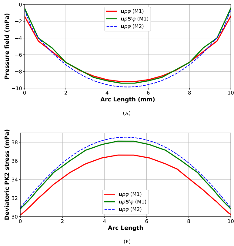
FIGURE 14 | Electrically induced bending plate. Comparison of the pressure field and the Frobenius norm of the deviatoric PK2 mechanical stress along segment A-A' for both up\phi and upS'\phi formulations at load increment \lambda = 0.9 . (a) Pressure field, (b) Deviatoric PK2 mechanical stress magnitude.
