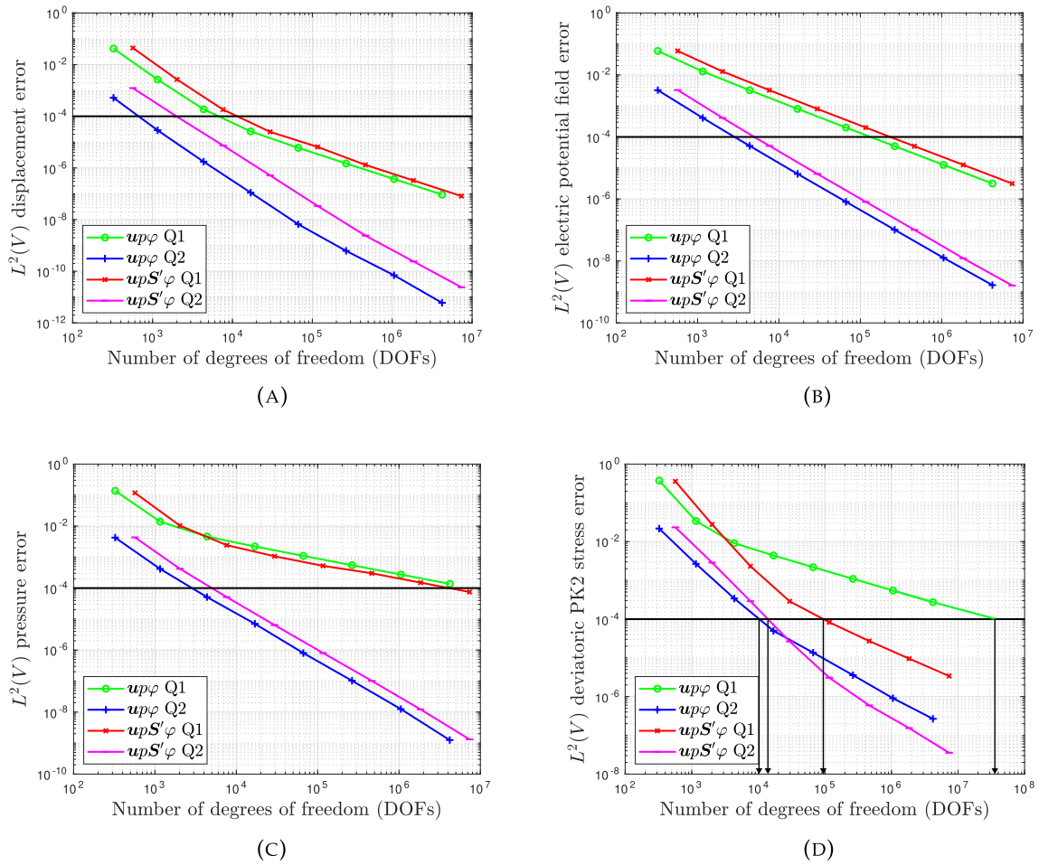
FIGURE 2 | Manufactured convergence test. Convergence rate for both up\phi and upS'\phi formulations upon DOFs. (a) Displacement error upon DOFs, (b) Electric potential error upon DOFs, (c) Pressure error upon DOFs, and (d) Deviatoric PK2 mechanical stress error upon DOFs.
