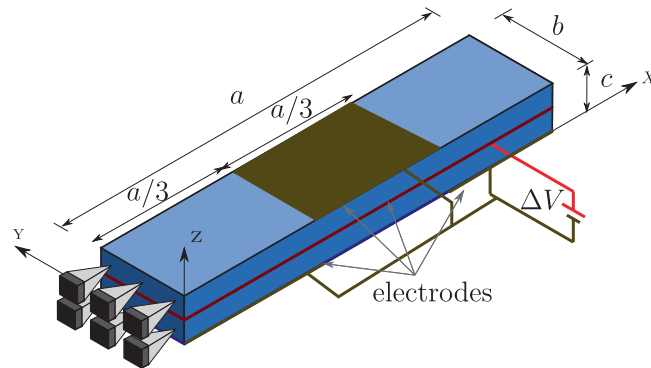
FIGURE 15 | Complex electrically induced bending plate. Geometry.
