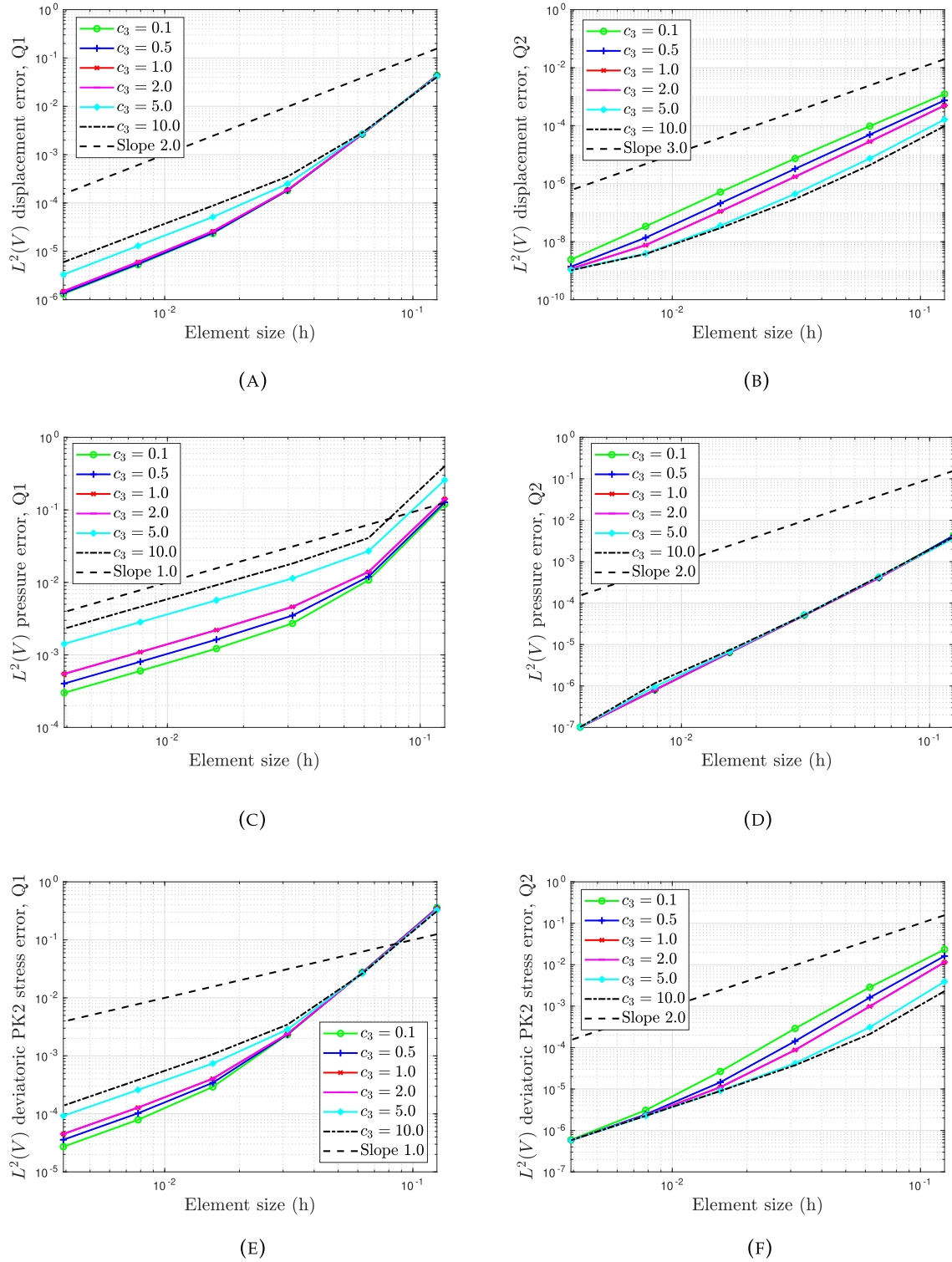
FIGURE 5 | Manufactured convergence test. Convergence rate for u\mathbf{p}\mathbf{S}'\boldsymbol{\varphi} formulation upon mesh refinement. Study to determine the optimal parameter c_3 . (a) Displacement error upon mesh refinement, Q1 elements, (b) Displacement error upon mesh refinement, Q2 elements, (c) Pressure error upon mesh refinement, Q1 elements, (d) Pressure error upon mesh refinement, Q2 elements, (e) Deviatoric PK2 mechanical stress error upon mesh refinement, Q1 elements, and (f) Deviatoric PK2 mechanical stress error upon mesh refinement, Q2 elements.
