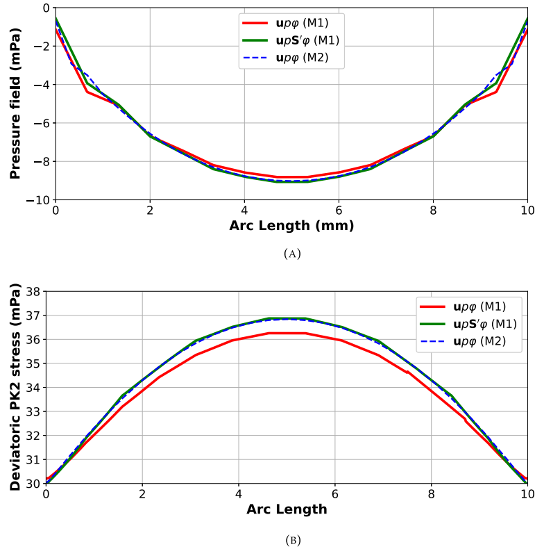
FIGURE 17 | Complex electrically induced bending plate. Comparison of the pressure field and the Frobenius norm of the deviatoric PK2 mechanical stress along segment A-A' for both up\phi and upS'\phi formulations at load increment \lambda = 0.66 . (a) Pressure field, (b) Deviatoric PK2 mechanical stress magnitude.
