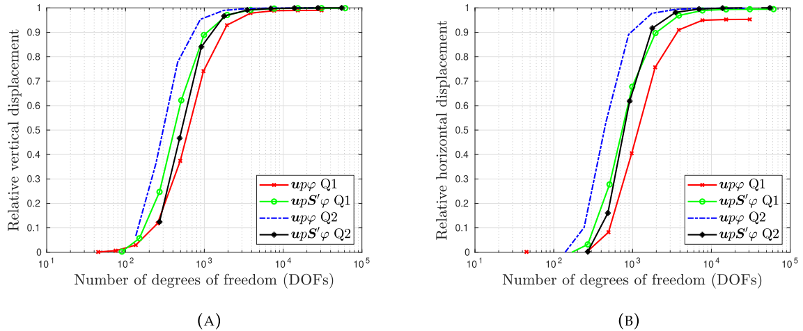
FIGURE 8 | Electrically induced bending beam. Displacement at point A for both up and ups formulations upon DOFs for AR = 100. (a) Relative vertical displacement upon DOFs, (b) Relative horizontal displacement upon DOFs.
