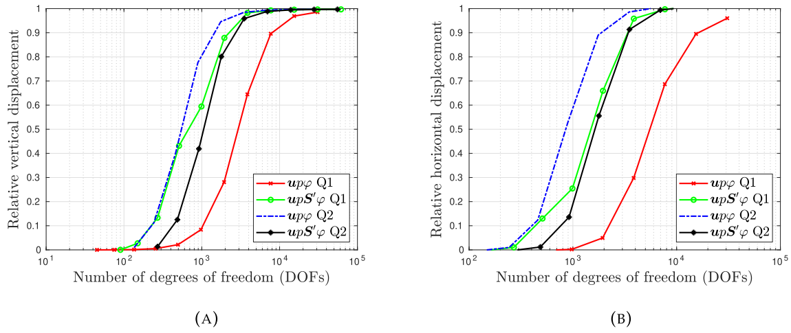
FIGURE 10 | Electrically induced bending beam. Displacement at point A for both up\phi and upS'\phi formulations upon DOFs for AR = 500 . (a) Relative vertical displacement upon DOFs, (b) Relative horizontal displacement upon DOFs.
