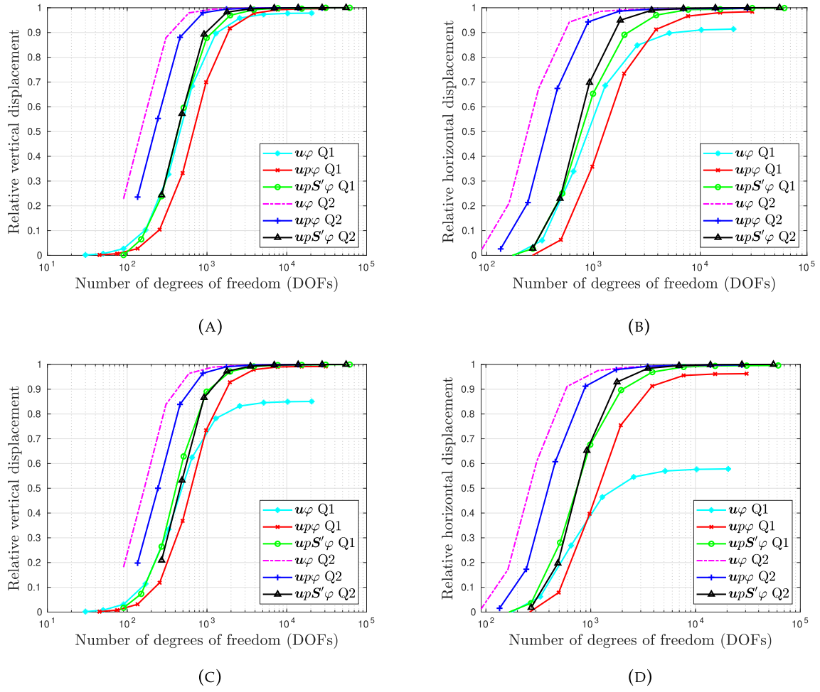
FIGURE 7 | Electrically induced bending beam. Displacement at point A for u\varphi , up\varphi and upS'\varphi formulations upon DOFs for AR = 100. (a) Relative vertical displacement upon DOFs, \nu = 0.45 , (b) Relative horizontal displacement upon DOFs, \nu = 0.45 , (c) Relative vertical displacement upon DOFs, \nu = 0.49 , and (d) Relative horizontal displacement upon DOFs, \nu = 0.49 .
