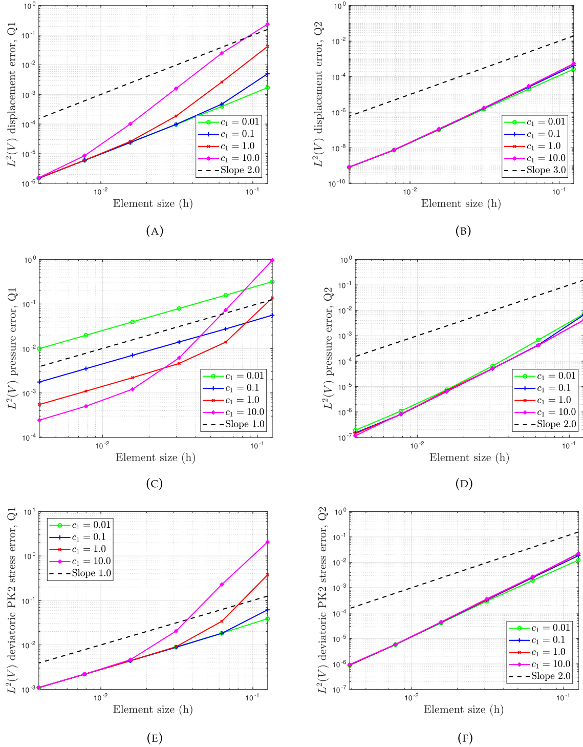
FIGURE 3 | Manufactured convergence test. Convergence rate for up\phi formulation upon mesh refinement. Study to determine the optimal parameter c_1 . (a) Displacement error upon mesh refinement, Q1 elements, (b) Displacement error upon mesh refinement, Q2 elements, (c) Pressure error upon mesh refinement, Q1 elements, (d) Pressure error upon mesh refinement, Q2 elements, (e) Deviatoric PK2 mechanical stress error upon mesh refinement, Q1 elements, and (f) Deviatoric PK2 mechanical stress error upon mesh refinement, Q2 elements.
