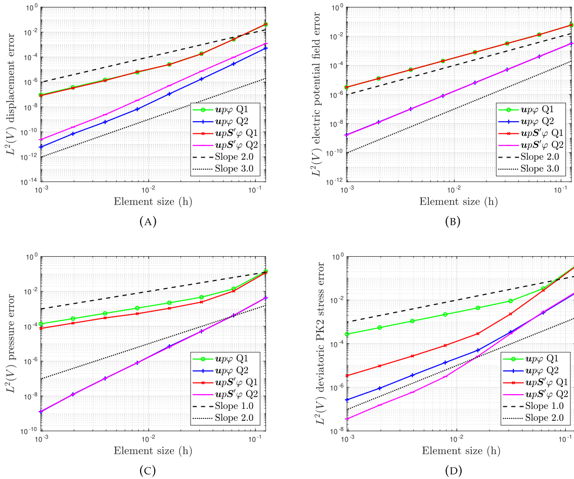
FIGURE 1 | Manufactured convergence test. Convergence rate for both up\varphi and upS'\varphi formulations upon mesh refinement. (a) Displacement error upon mesh refinement, (b) Electric potential error upon mesh refinement, (c) Pressure error upon mesh refinement, and (d) Deviatoric PK2 mechanical stress error upon mesh refinement.
