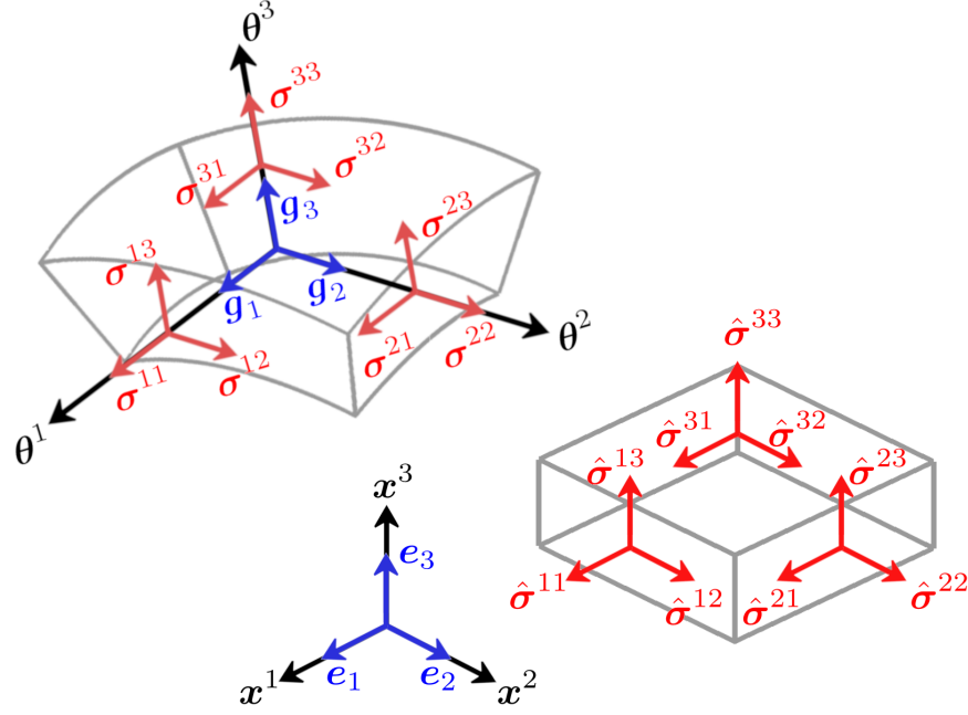
Figure 1: Notation for the stress components. In curvilinear coordinates, the stresses can be grouped as follows: \sigma^{11} , \sigma^{22} are the membrane stresses; \sigma^{12} = \sigma^{21} are the twisting stresses; \sigma^{13} = \sigma^{31} , \sigma^{23} = \sigma^{32} are the shear stresses; \sigma^{33} is the transverse stress. In Cartesian coordinates, this physical interpretation is not possible.
