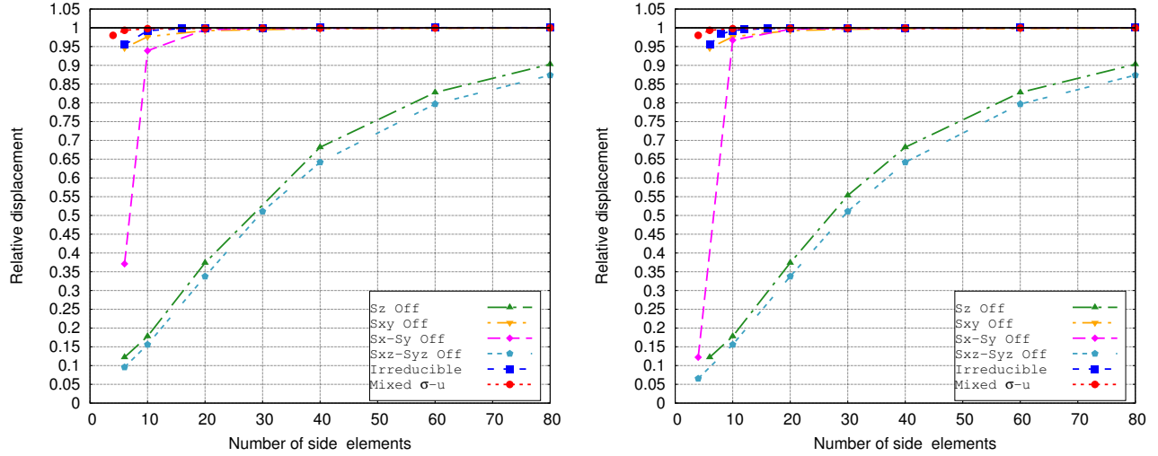
Figure 13: Scordelis-Lo roof: Stress deactivation convergence curves using n_{\text{nelem}} = 2 (left) and n_l = 2 (right).
