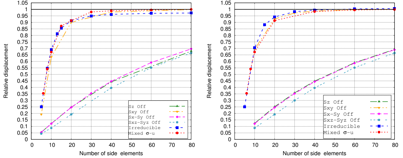
Figure 22: Pinched cylinder: Stress deactivation convergence curves using n_{nelem} = 2 (left) and n_l = 2 (right).
