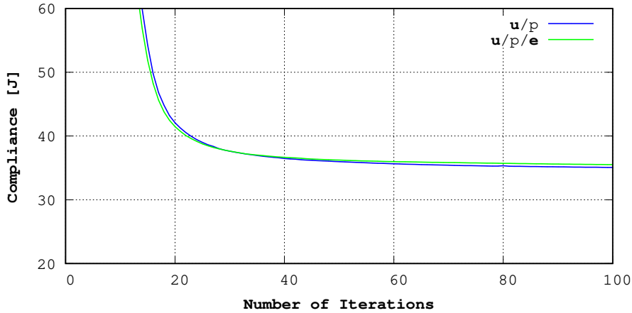
FIGURE 8. Single-point load beam. Convergence diagrams in plane strain scenario for \nu_s = 0.5 for both \mathbf{u}/p and \mathbf{u}/p/e formulations.
