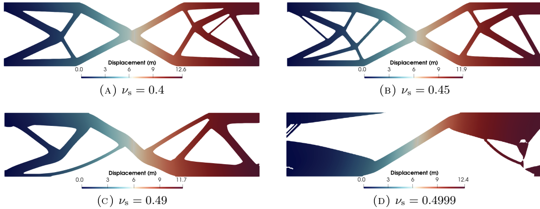
FIGURE 4. Single-point load beam. Final optimized structure in plane strain scenario while increasing the incompressibility of the stiff material.
