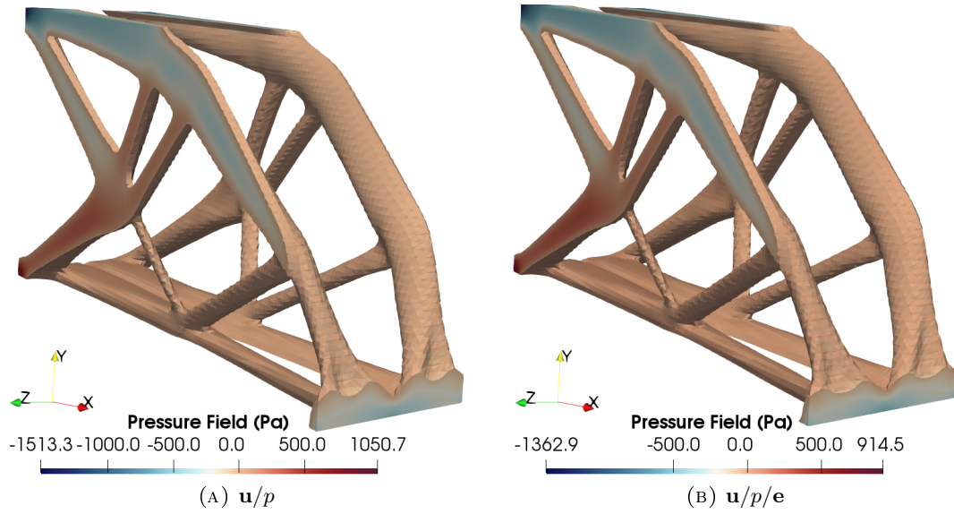
FIGURE 19. 3D Cantilever beam. Pressure field for the optimized structure in a 3D scenario for \nu_s = 0.5 .
