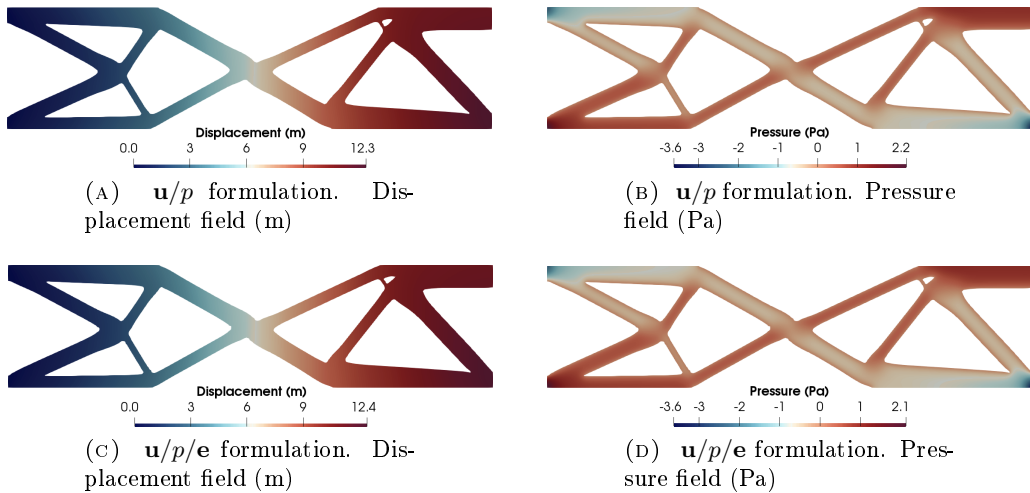
FIGURE 7. Single-point load beam. Final optimized structure in plane strain scenario for \nu_s = 0.5 for both \mathbf{u}/p and \mathbf{u}/p/e formulations.
