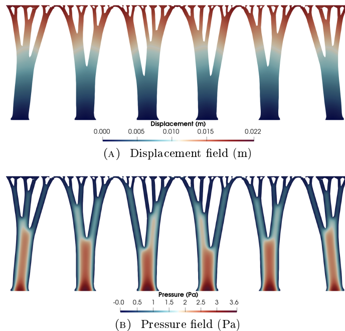
FIGURE 11. Bearing device. Final optimized structure in plane strain scenario for \nu_s = 0.5 and \nu_w = 0.4 for \mathbf{u}/p formulation.
