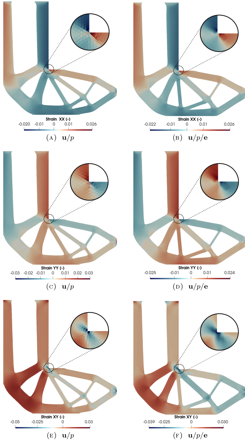
FIGURE 16. L-shaped beam. Deviatoric strain field for the optimized structure for \nu_s = 0.5
