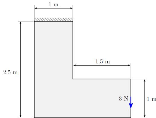
FIGURE 13. L-shaped beam. Geometry.
