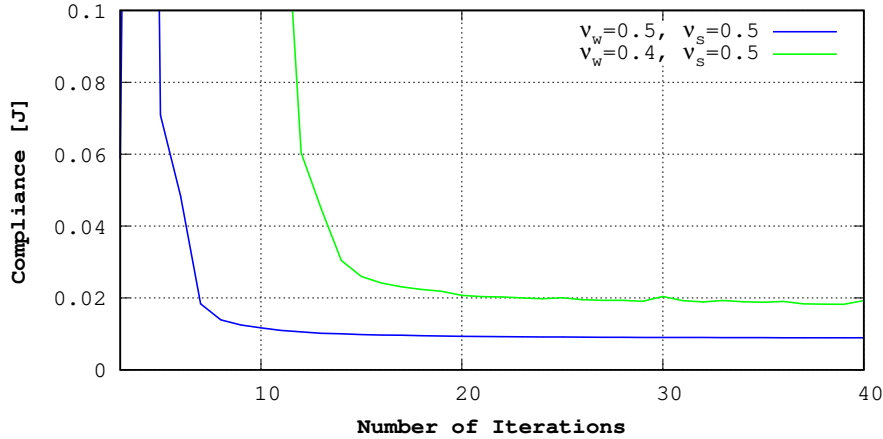
FIGURE 12. Bearing device. Convergence diagrams in plane strain scenario for \mathbf{u}/p formulation considering both \nu_w = 0.4 and \nu_w = 0.5 .
