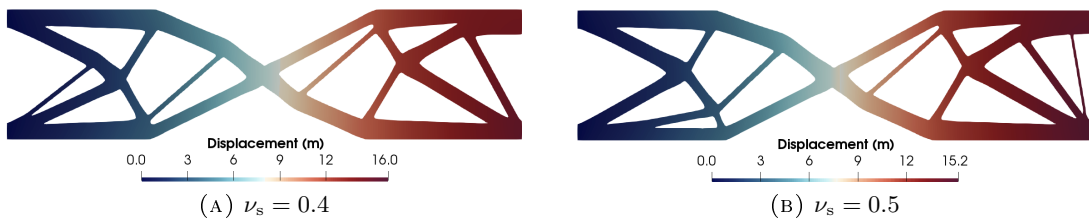
FIGURE 3. Single-point load beam. Final optimized structure in plane stress scenario.
