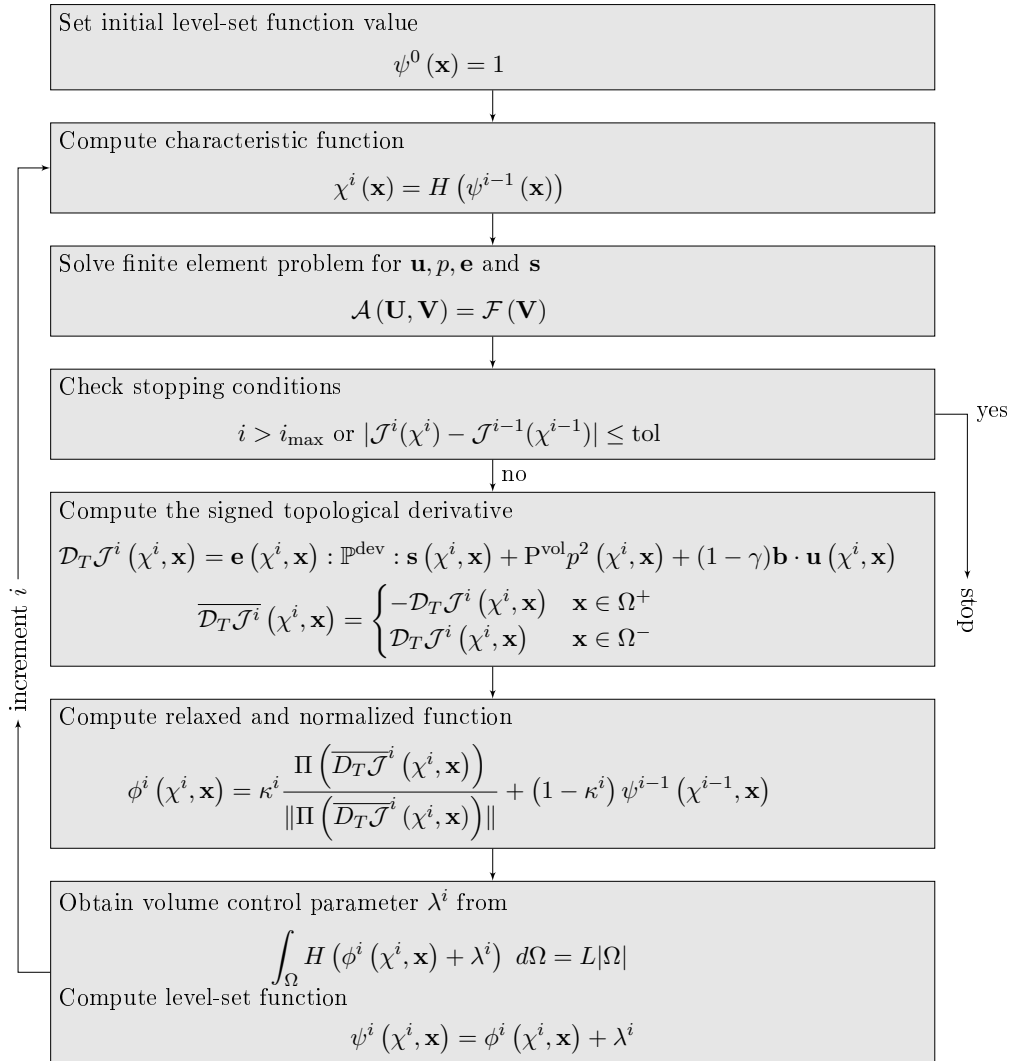
FIGURE 1. Topology Optimization Algorithm Flowchart
