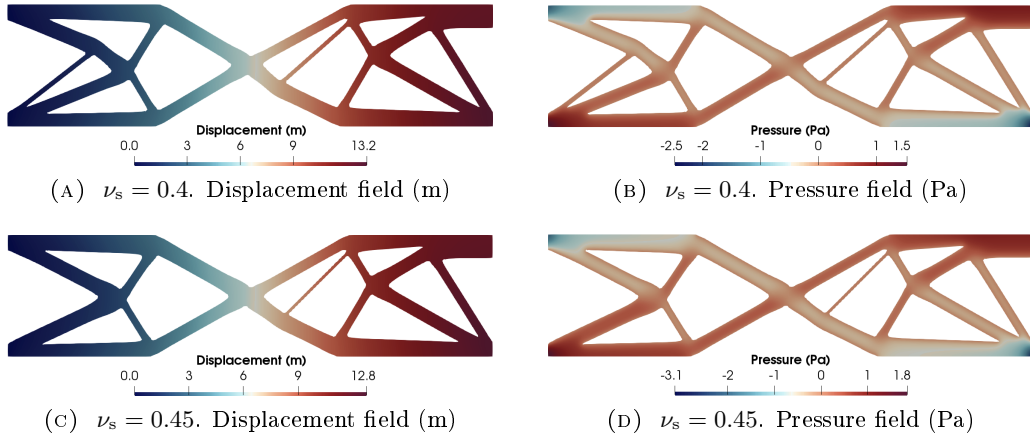
FIGURE 6. Single-point load beam. Final optimized structure in plane strain scenario for compressible materials with \mathbf{u}/p/e formulation.
