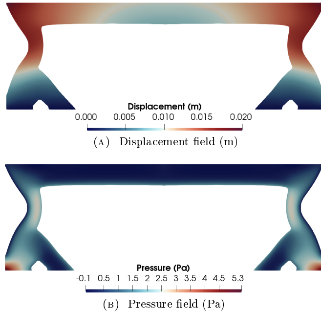
FIGURE 10. Bearing device. Final optimized structure in plane strain scenario for \nu_s = 0.5 and \nu_w = 0.5 for \mathbf{u}/p formulation.
