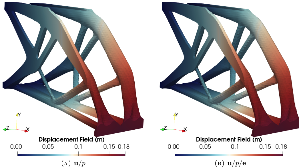
FIGURE 18. 3D Cantilever beam. Displacement field for the optimized structure in a 3D scenario for \nu_s = 0.5 .
