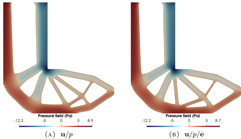
FIGURE 15. L-shaped beam. Pressure field for the optimized structure for \nu_s = 0.5
