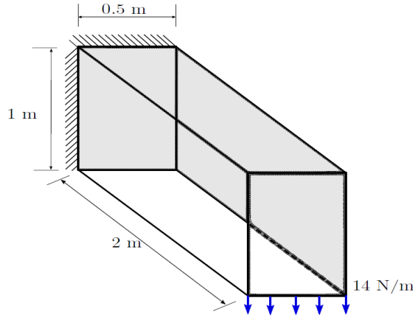
FIGURE 17. 3D Cantilever beam. Geometry.
