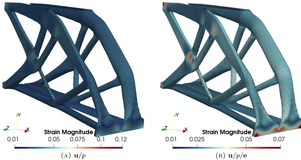
FIGURE 20. 3D Cantilever beam. Deviatoric strain field magnitude for the optimized structure in a 3D scenario for \nu_s = 0.5 .
