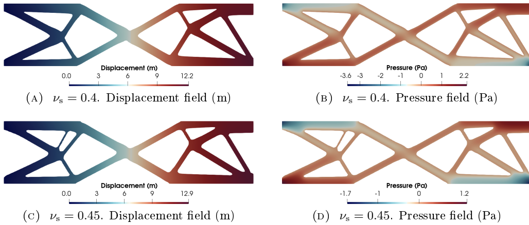
FIGURE 5. Single-point load beam. Final optimized structure in plane strain scenario for compressible materials with \mathbf{u}/p formulation.
