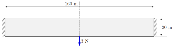
FIGURE 2. Single-point load beam. Geometry
