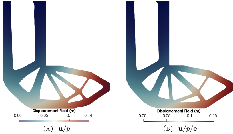
FIGURE 14. L-shaped beam. Displacement field for the optimized structure for \nu_s = 0.5
