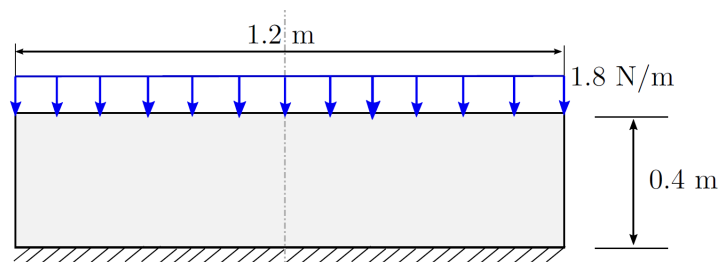
FIGURE 9. Bearing device. Geometry
