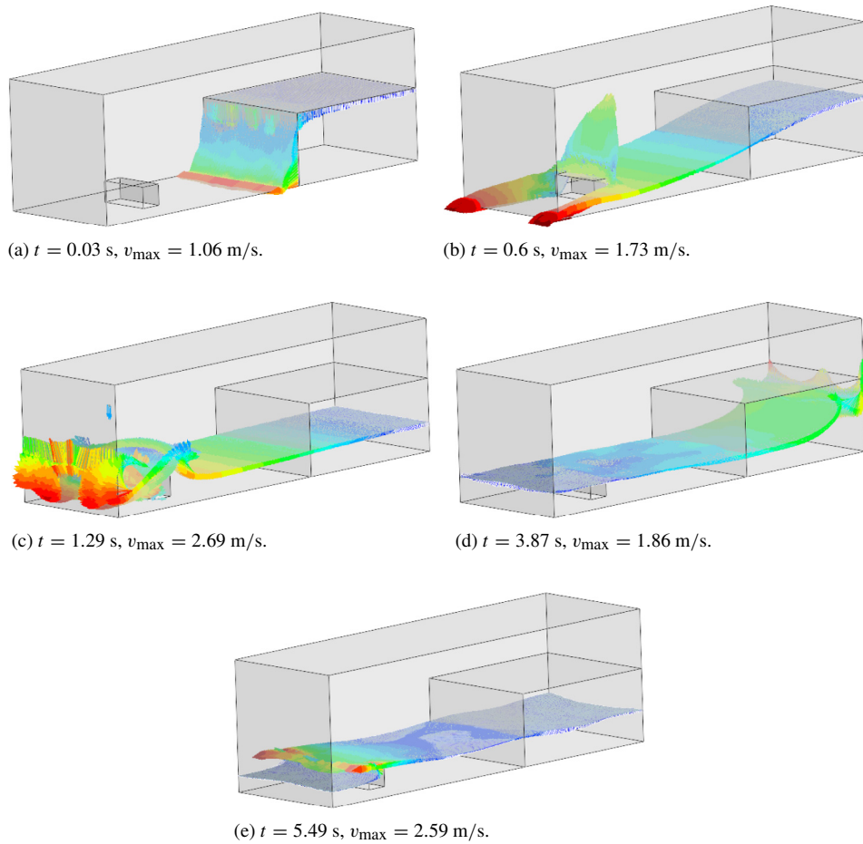
Fig. 22. Velocity vectors at the free surface for the dam-break problem at several time steps. Vector colors indicate velocity magnitudes (with light red indicating the maximum velocity, dark blue indicating fluid at rest), vector arrowheads indicate flow direction. The maximum fluid nodal velocity at each time step is indicated in the captions. (For interpretation of the references to colour in this figure legend, the reader is referred to the web version of this article.)
