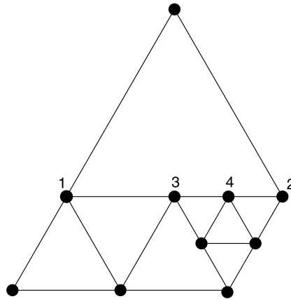
Fig. 5. Hanging nodes. Node 4 is a hanging node, its hanging parents being nodes 2 and 3. Node 3 is in turn a hanging node, its hanging parents being nodes 1 and 2. The hanging node value for the unknown at node 4, u_4 is: u_4 = \frac{1}{2}u_3 + \frac{1}{2}u_2 = \frac{1}{4}u_1 + \frac{3}{4}u_2 .
