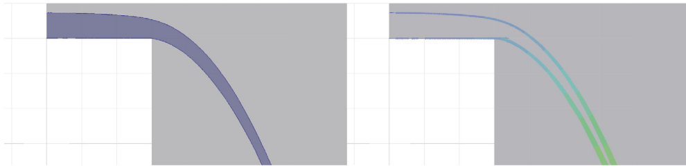
Fig. 16. Free falling jet problem. Left: free surface plot. Right: Velocity vector field when the stationary state is reached. Vector colors indicate velocity magnitude, vector arrowheads indicate direction. (For interpretation of the references to colour in this figure legend, the reader is referred to the web version of this article.)
