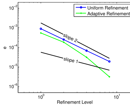
Fig. 7. Spatial convergence for the 2D sloshing in a rectangular tank.
