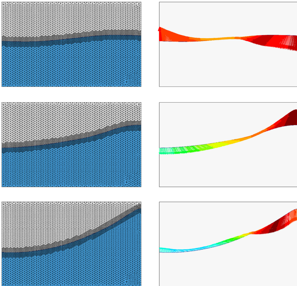
Fig. 13. Mesh and position of the free surface (left) and velocity vectors (right) at several time instants of the simulation. Vector colors indicate velocity magnitudes, vector arrowheads indicate velocity direction. (For interpretation of the references to colour in this figure legend, the reader is referred to the web version of this article.)
