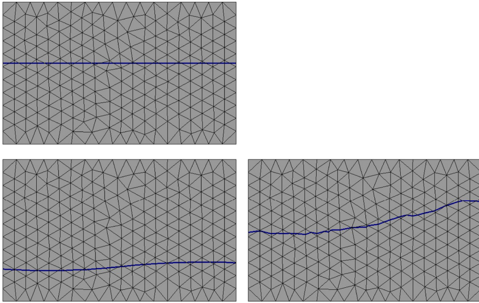
Fig. 10. Effect of the mass loss correction scheme. Top: Initial level set configuration. Bottom: Level set position at the end of the simulation without (left) and with (right) mass loss correction scheme.
