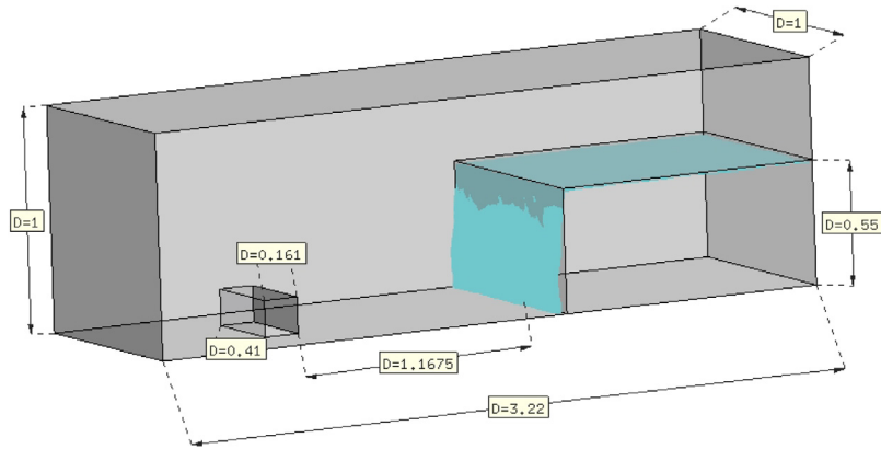
Fig. 19. Kleefman's dambreaking experiment initial configuration.
