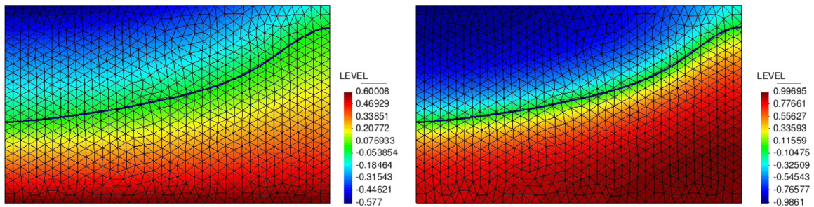
Fig. 11. Effect of the level set reinitialization scheme. Left: Without reinitialization. Right: With reinitialization.
