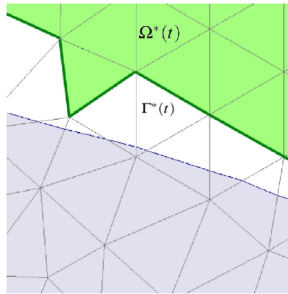
Fig. 3. Definition of \Omega^*(t) and \Gamma^*(t) (in green) for the harmonic extension of u_h and p_h into \Omega^0 \setminus \Omega(t) . (For interpretation of the references to colour in this figure legend, the reader is referred to the web version of this article.)
