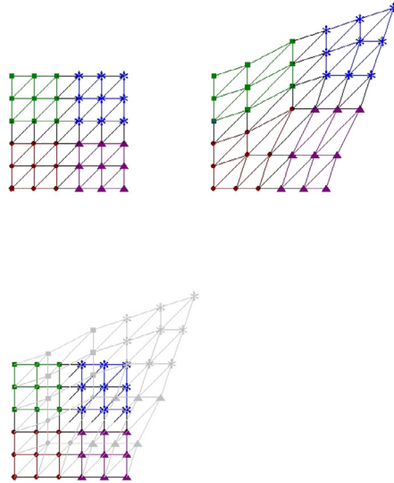
Fig. 4. Projection from the deformed to the background mesh. Top left: original mesh. Top right: deformed mesh. Bottom left: projection process. Four different processors and subdomains exist in this case. In the bottom left image, the projection from the deformed to the background mesh is performed. Some nodes lay in the same processor for the deformed and the undeformed mesh (top left square green nodes, for instance). Other nodes however, need information from a different processor in order to do the projection step. This is the case of the bottom left central blue star node, which needs to be interpolated from the bottom-left red domain. Inter-processor communications are required in this case.
