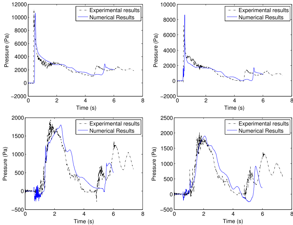
Fig. 21. Comparison of experimental and numerical values for the pressure time history at several points of the obstacle surface (P1 to P4). From left to right and then top to bottom: P1: (0.8245, 0.021, 0.4965), P2: (0.8245, 0.141, 0.4965), P3: (0.7635, 0.161, 0.4965), P4: (0.7235, 0.161, 0.4965).
