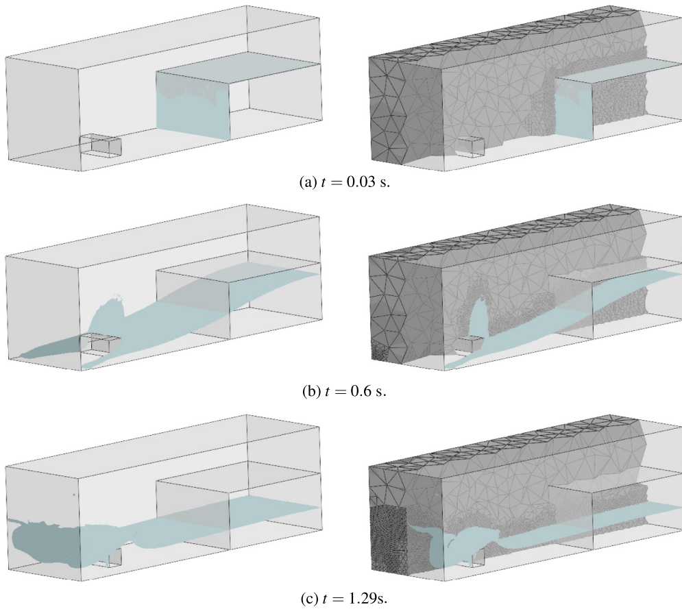
Fig. 20. Position of the free surface and computational mesh at several instants of the simulation for the green water flow case.
