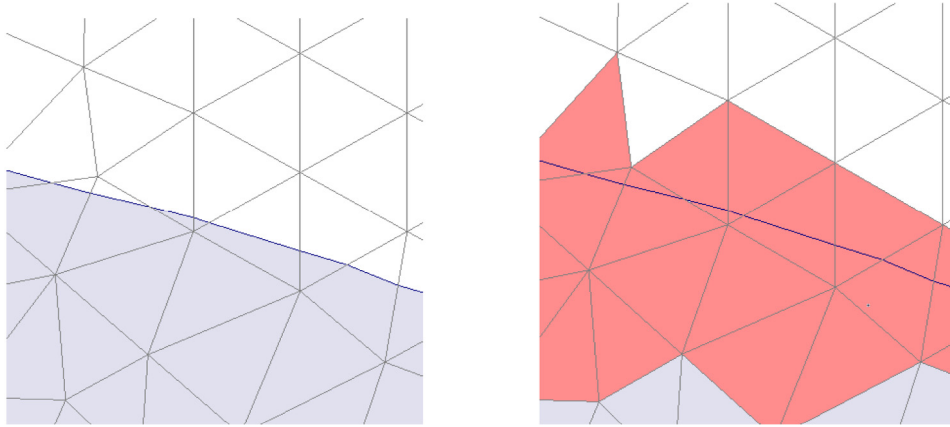
Fig. 2. Left: Free surface cuts causing ill-conditioning on the final linear system of equations. Right: Definition of the domain \Omega_{\text{cut}}(t) (in orange) used to integrate the ghost penalty stabilization terms. (For interpretation of the references to colour in this figure legend, the reader is referred to the web version of this article.)
