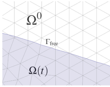
Fig. 1. Background domain \Omega^0 , and fixed background mesh. The domain covered by the fluid \Omega(t) (in blue) evolves in time. The free surface boundary \Gamma_{\text{free}} cuts some elements of the mesh in an arbitrary manner. This introduces the need for integrating the finite element equations only on the region covered by \Omega(t) in these elements, leading to subintegration. (For interpretation of the references to colour in this figure legend, the reader is referred to the web version of this article.)
