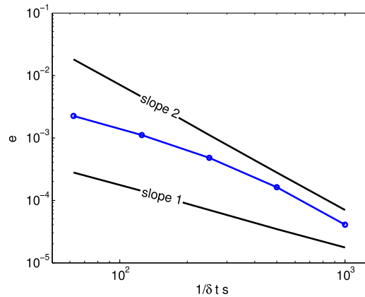
Fig. 8. Temporal convergence for the 2D sloshing in a rectangular tank.
