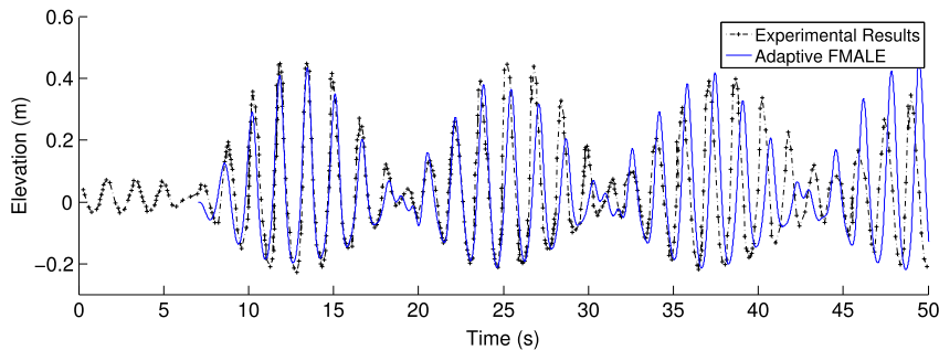
Fig. 15. Water surface elevation at an elevation gauge situated at x = 0.05 , z = 0.1 .
