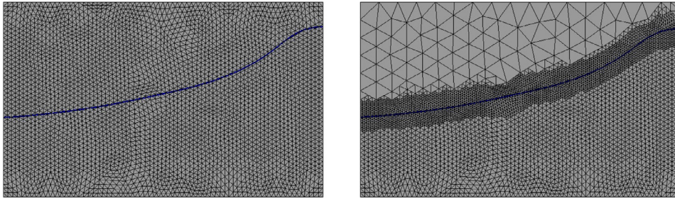
Fig. 6. Uniformly refined mesh (left) and adaptively refined mesh (right) used for the convergence study in the 2D sloshing tank.
