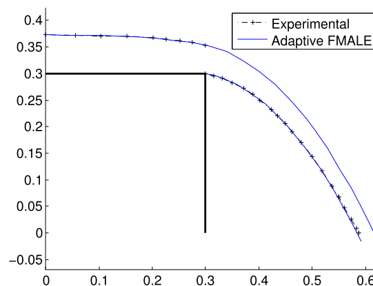
Fig. 18. Comparison of experimental and numerical simulation results for the free falling jet problem.
