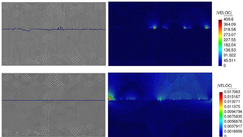
Fig. 9. Effect of the ghost penalty stabilization terms. Top: Result without the ghost penalty stabilization terms for a bad cut configuration. Bottom: Results with the ghost penalty stabilization terms.
