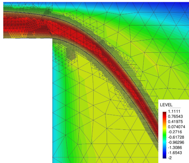
Fig. 17. Free falling jet problem. Adaptively refined mesh and level set function field when the stationary state is reached.
