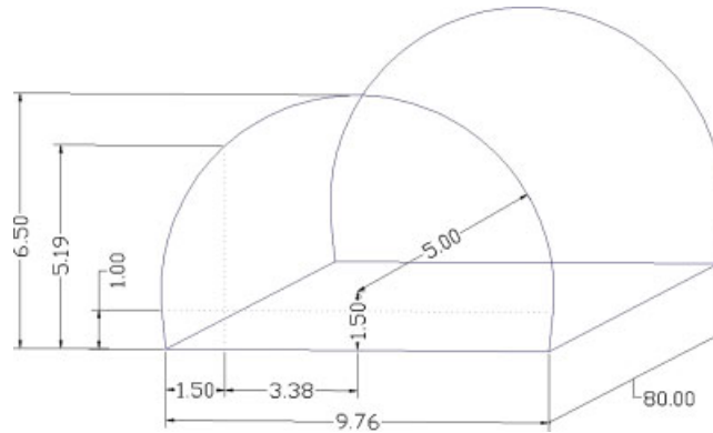
Figure 2. Geometry of the 3D fluid domain.
