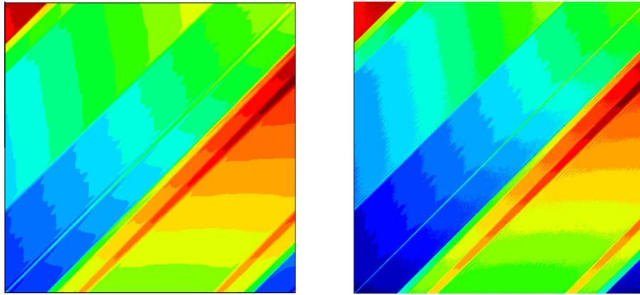
Fig. 5. Radiative intensity solution using the SUPG (left) and the Galerkin (right) methods in a mesh of 480 \times 480 elements. Case 2 ( \kappa = 0.01 \text{ m}^{-1} and \sigma_s = 0.001 \text{ m}^{-1} ).
