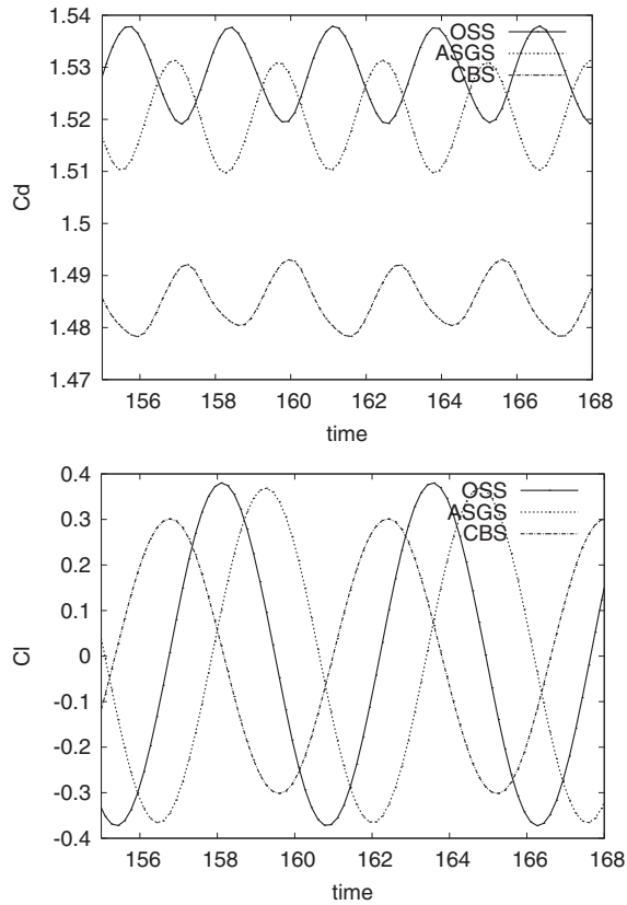
Figure 11. C_D and C_L for a flow around a cylinder at Re = 100 .
