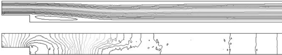
Figure 7. Streamline and pressure pattern for the BFS flow problem at Reynolds 229 using mesh 2 and the ASGS method.
