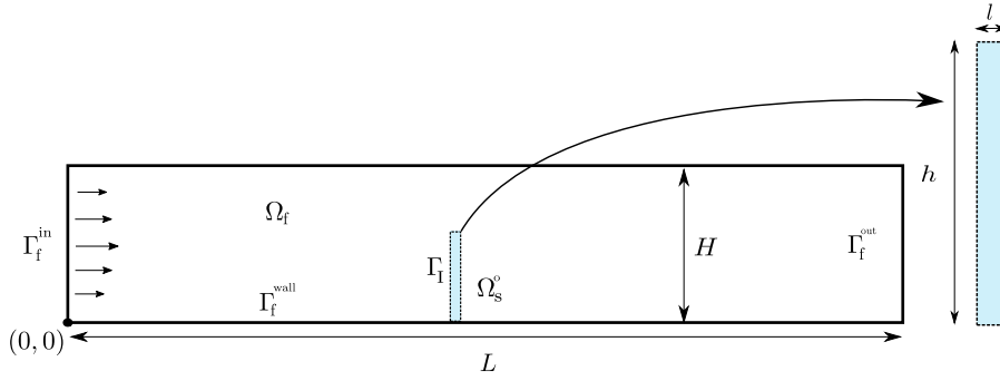
Fig. 2. Flow through a channel with a flexible flap. Geometry.
