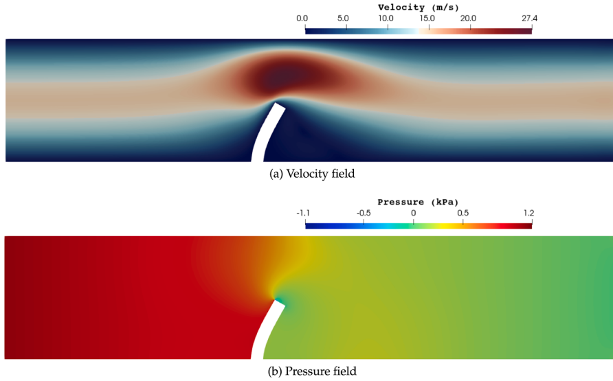
Fig. 3. Flow through a channel with a flexible flap. Distribution of the velocity field (top) and pressure (bottom) in the fluid domain for the stationary solution. Velocities are plotted using their Euclidean norm.
