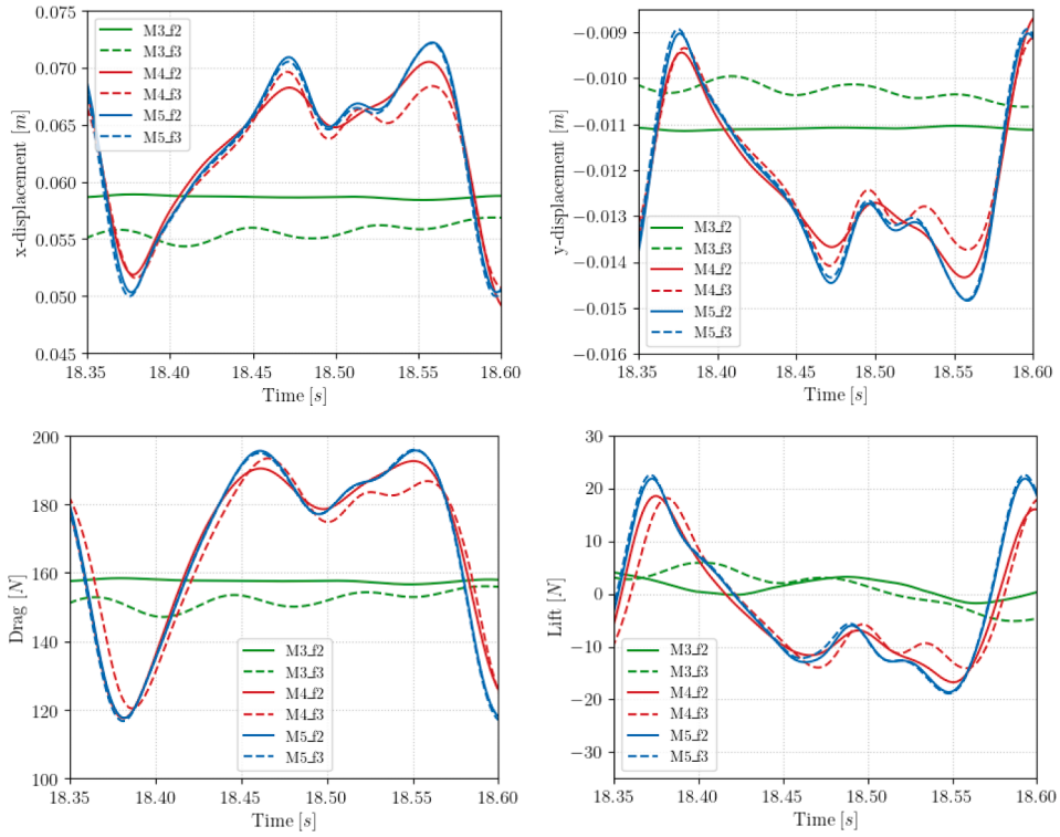
Fig. 7. Flow through a channel with a flexible flap. One period of the oscillatory solution at Re = 1000 .
