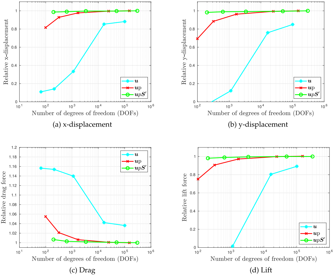
Fig. 6. Flow through a channel with a flexible flap. Comparative study for the solid formulations with respect to DOFs for a nearly incompressible material.
