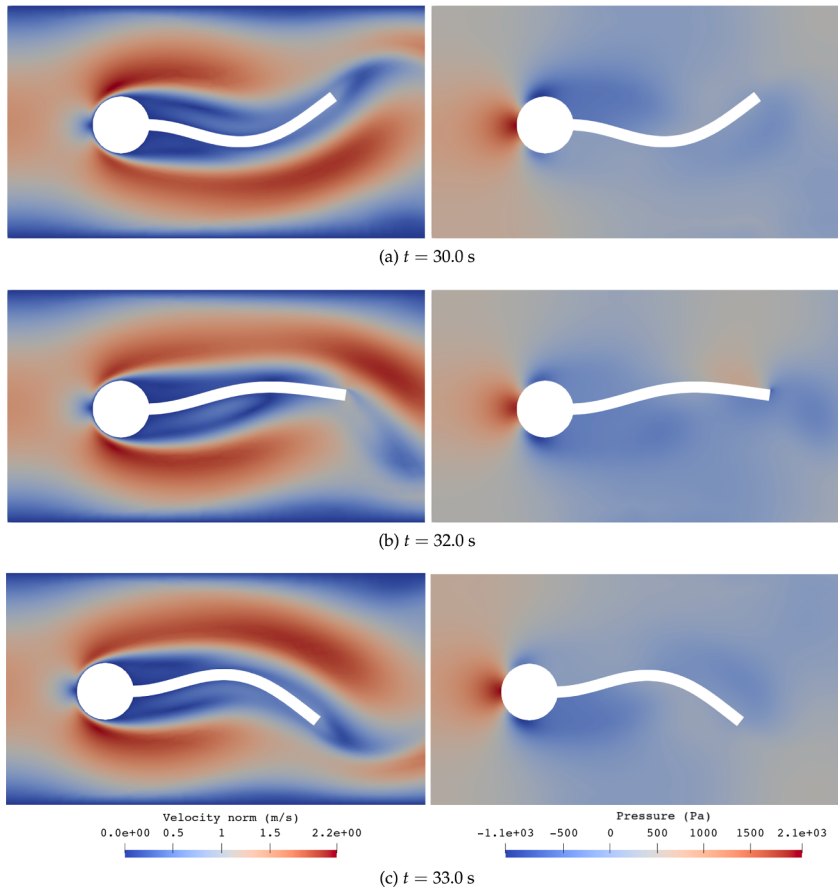
Fig. 11. Turek's test. Plot of the velocity norm and pressure for test FSI2 at different time instants.
