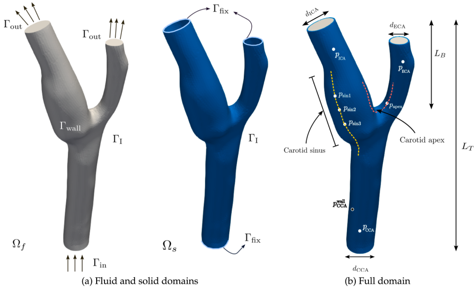
Fig. 13. Carotid blood flow. Geometry of the carotid artery bifurcation.
