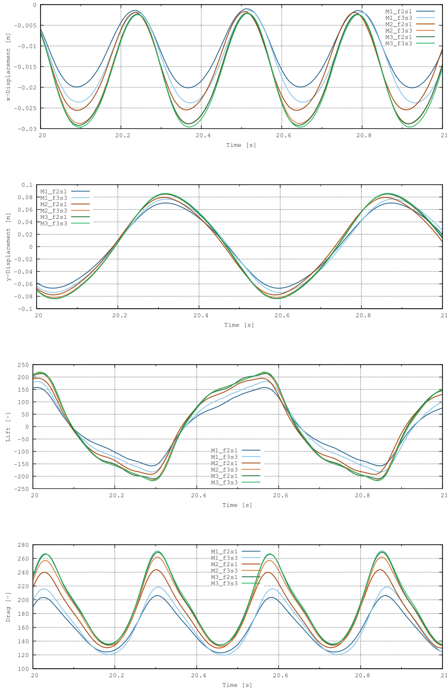
Fig. 12. Turek's test. Displacement at point A and drag and lift forces over the interface boundary \Gamma_I .
