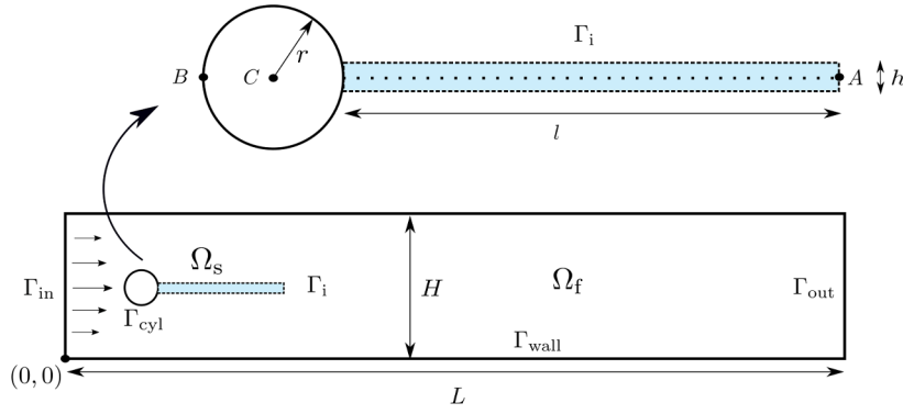
Fig. 9. Turek's test. Geometry.
