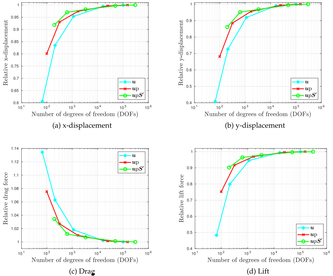
Fig. 4. Flow through a channel with a flexible flap. Comparative study for the solid formulations with respect to DOFs.
