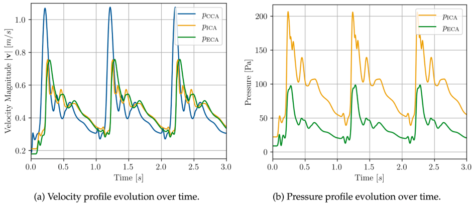
Fig. 18. Carotid blood flow. Temporal evolution of velocity and pressure profiles near the inlet and outlet regions.
