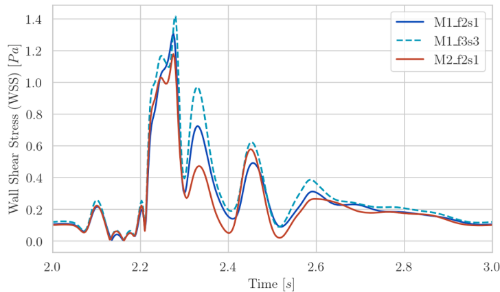
Fig. 24. Carotid blood flow. Evolution in time of the WSS in point p_{apex} .
