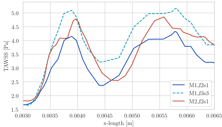
Fig. 23. Carotid blood flow. TAWSS comparison on the carotid surface apex.
