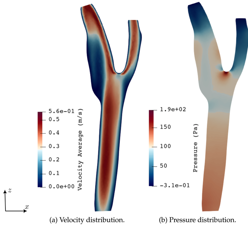
Fig. 17. Carotid blood flow. Time-averaged flow distribution in a cross-sectional view, represented in the reference configuration domain.
