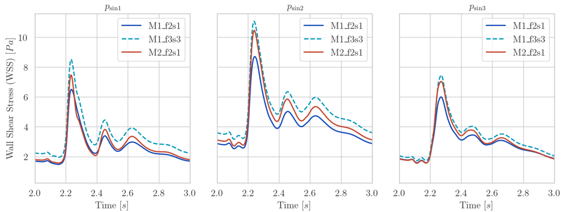
Fig. 21. Carotid blood flow. Evolution in time of the WSS in points ( p_{sin1} , p_{sin2} and p_{sin3} ) located over the sinus region.
