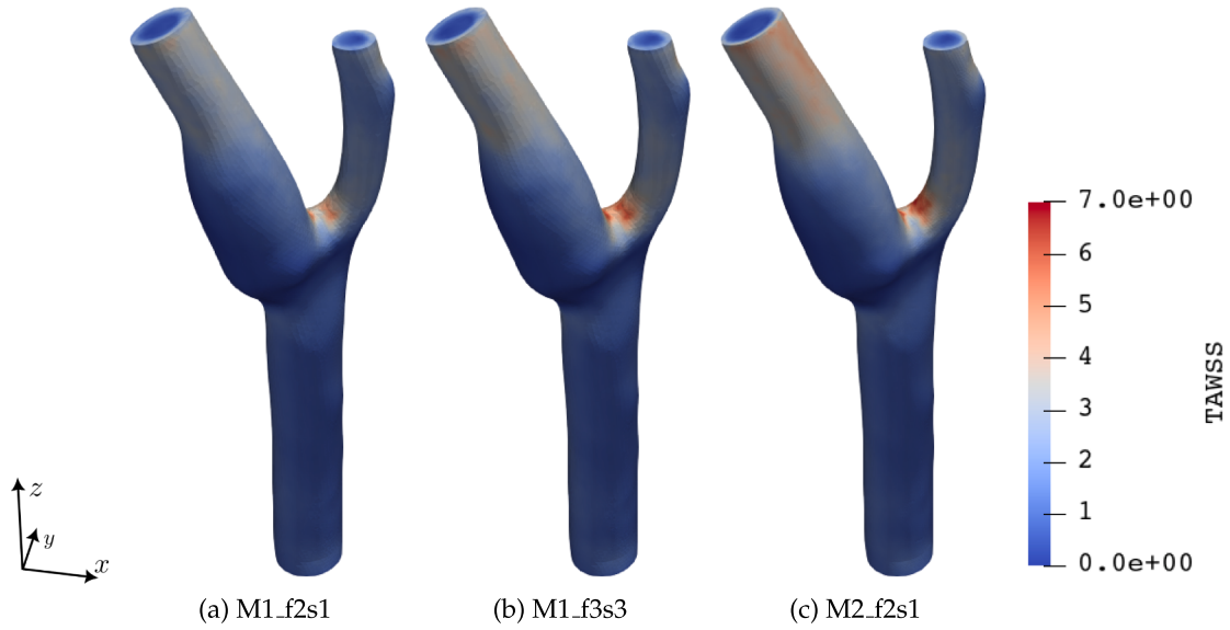
Fig. 22. Carotid blood flow. TAWSS distribution on the carotid surface for the three configurations.
