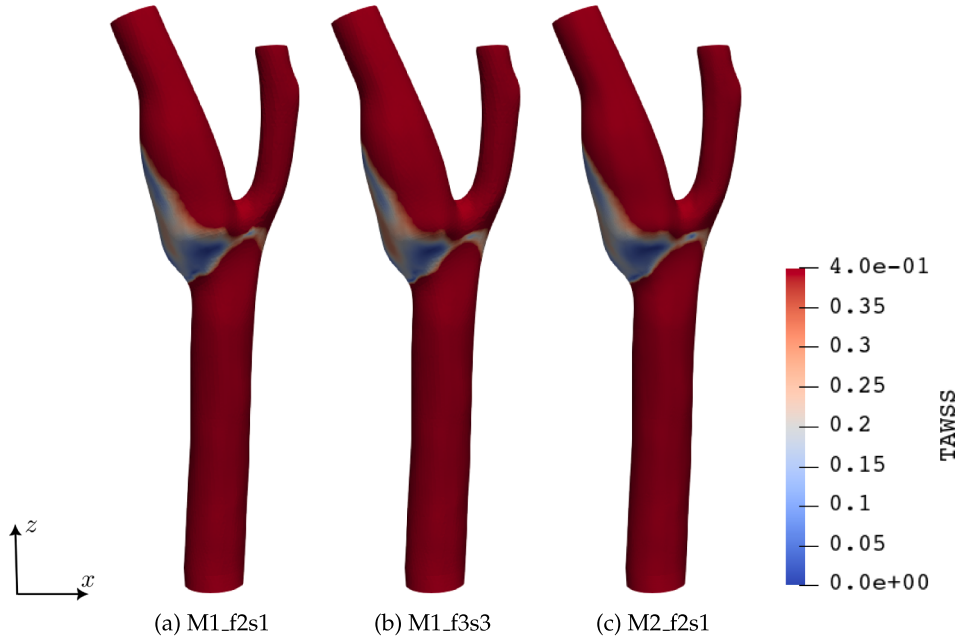
Fig. 19. Carotid blood flow. TAWSS distribution on the carotid surface sinus for the three configurations.
