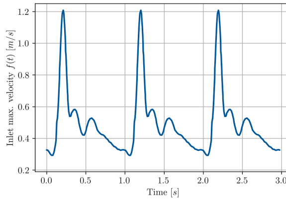
Fig. 14. Carotid blood flow. Evolution of the inlet velocity.
