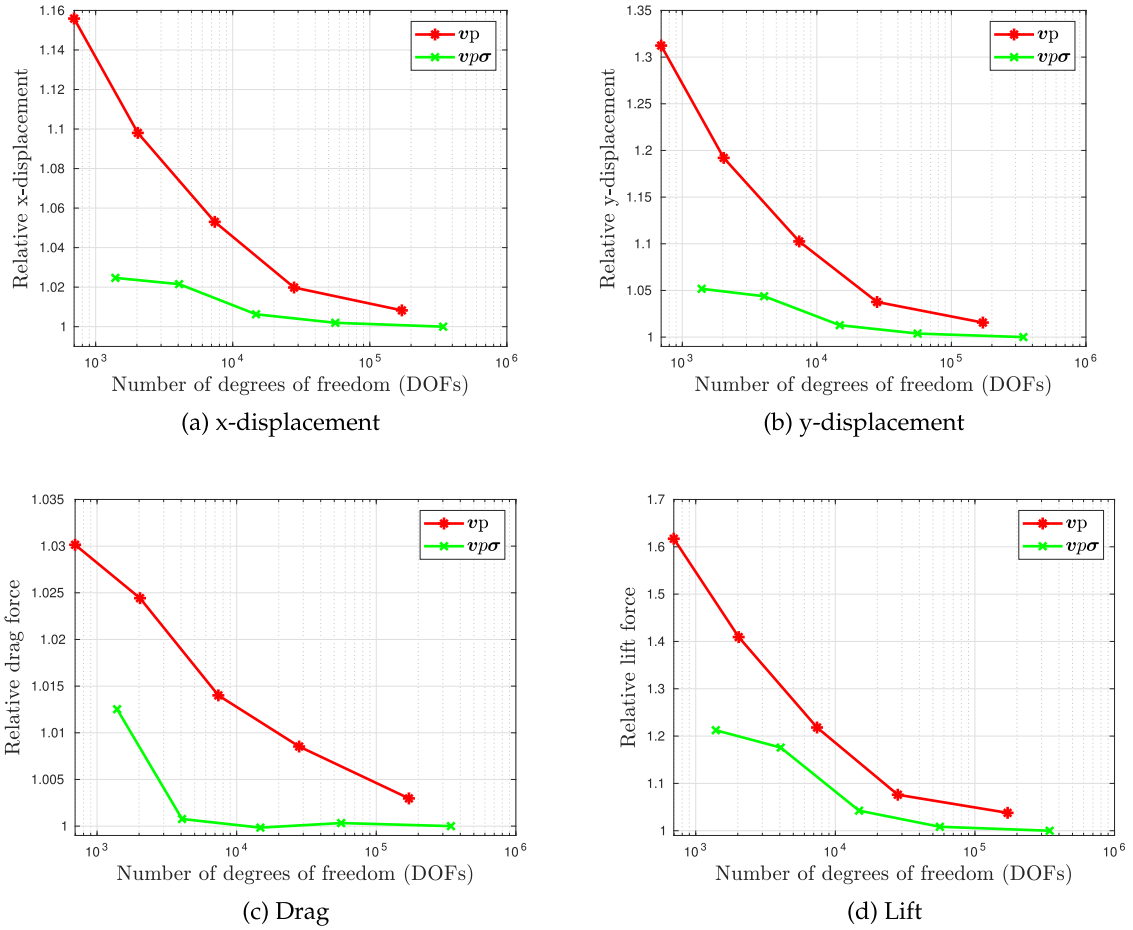
Fig. 5. Flow through a channel with a flexible flap. Comparative study for the fluid formulations with respect to DOFs.
