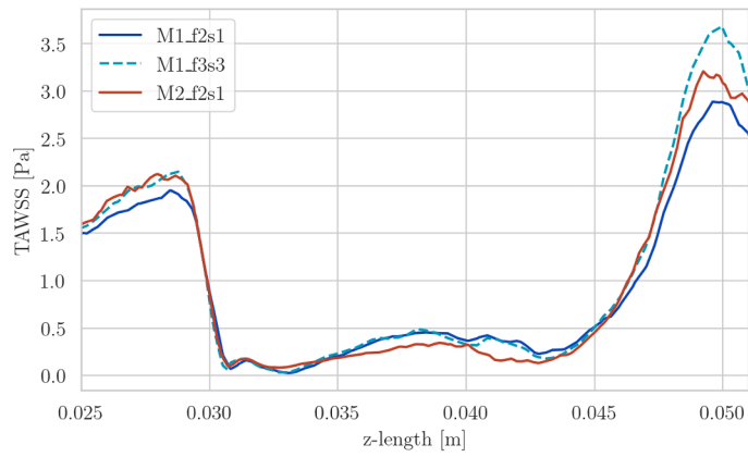
Fig. 20. Carotid blood flow. WSS comparison on the carotid surface sinus.
