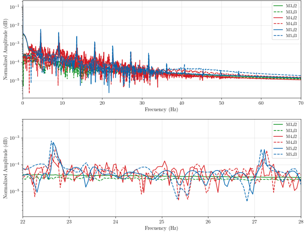
Fig. 8. Flow through a channel with a flexible flap. Fourier transform of the x-displacements at Re = 1000 .
