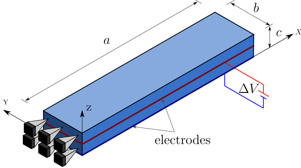
FIGURE 12. Electrically induced bending plate. Geometry.
