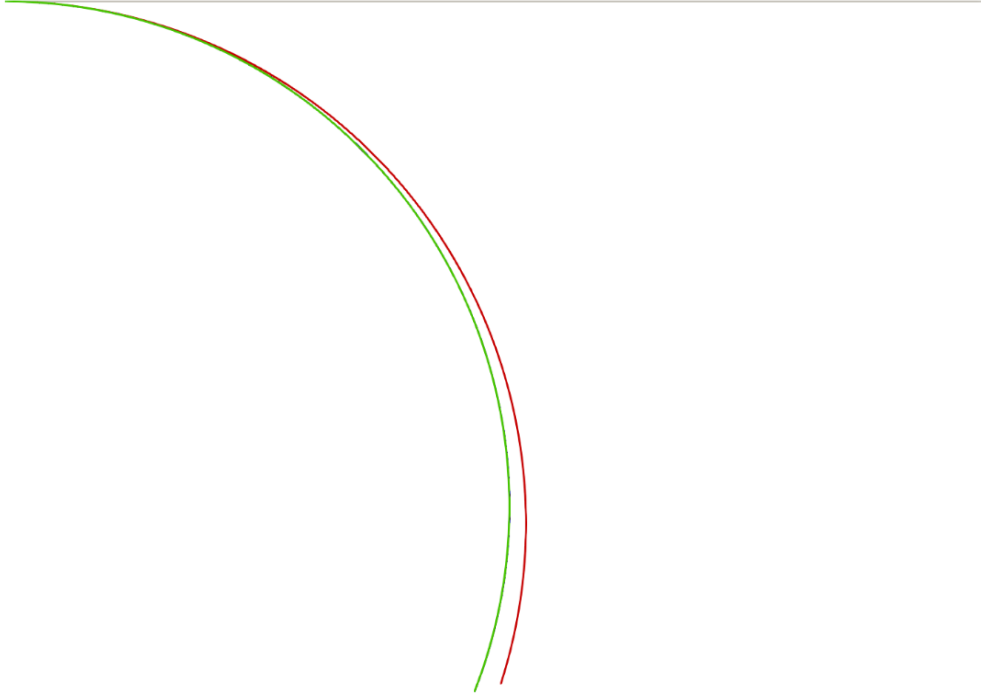
FIGURE 10. Electrically induced bending beam. Deformation of the beam for AR=500 using the finest mesh with N = 2048 FEs along the length. up\varphi Q1 (red), up\varphi Q2 (blue), upS'\varphi Q1 (green), upS'\varphi Q2 (black).
