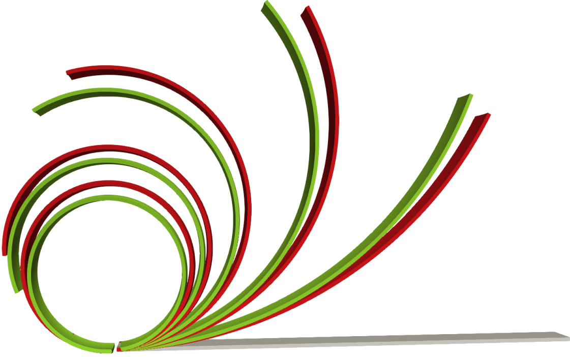
FIGURE 13. Electrically induced bending plate. Deformation of the plate for several load increments using mesh M1. up\varphi (red) and upS'\varphi (green) formulations.
