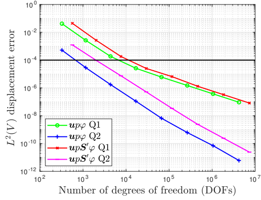
(A) Displacement error upon DOFs
