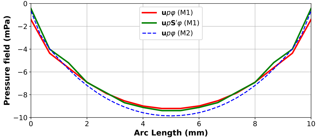
(A) Pressure field
