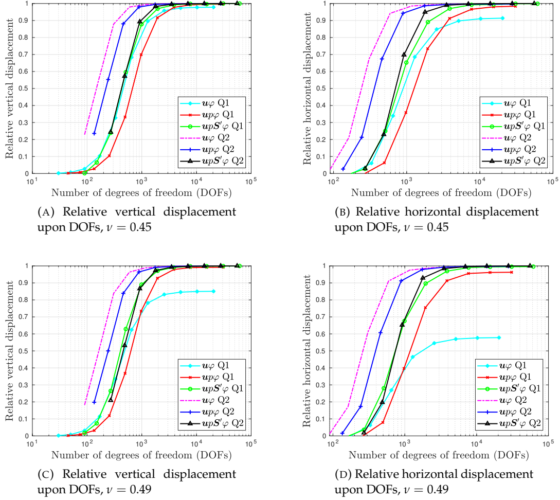
FIGURE 7. Electrically induced bending beam. Displacement at point A for u\varphi , up\varphi and upS'\varphi formulations upon DOFs for AR = 100 .
