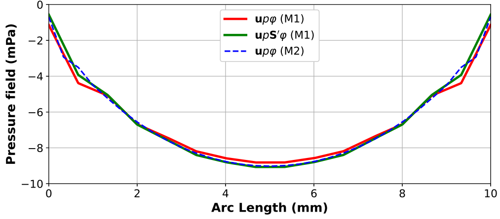
(A) Pressure field
