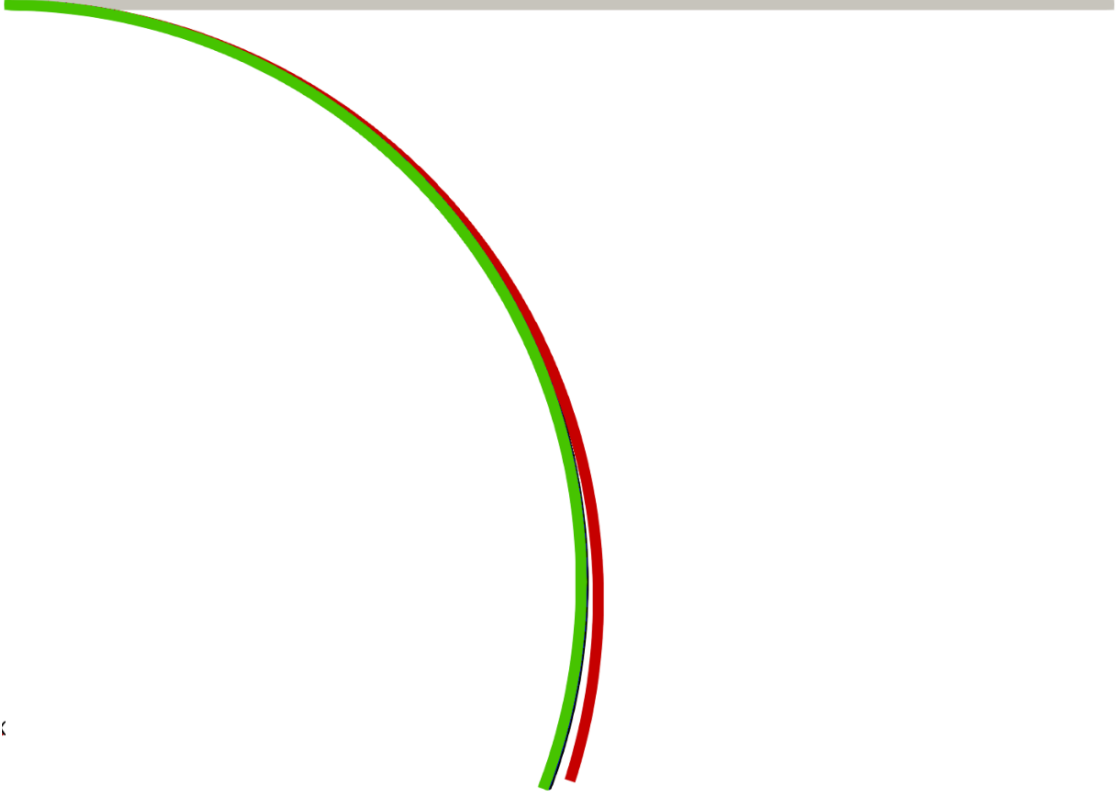
FIGURE 8. Electrically induced bending beam. Deformation of the beam for AR = 100 , using the finest mesh with N = 2048 FEs along the length. up\varphi Q1 (red), up\varphi Q2 (blue), upS'\varphi Q1 (green), upS'\varphi Q2 (black).
