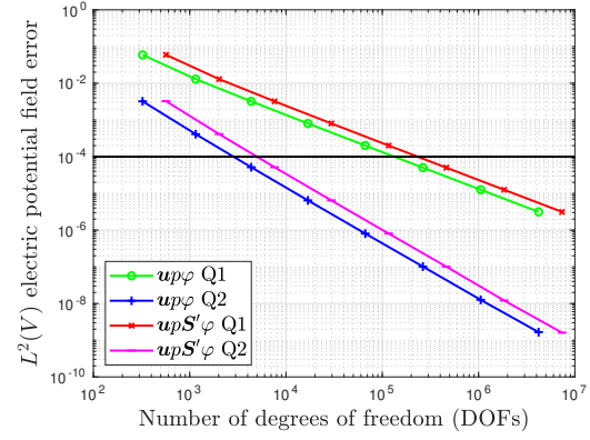
(B) Electric potential error upon DOFs
