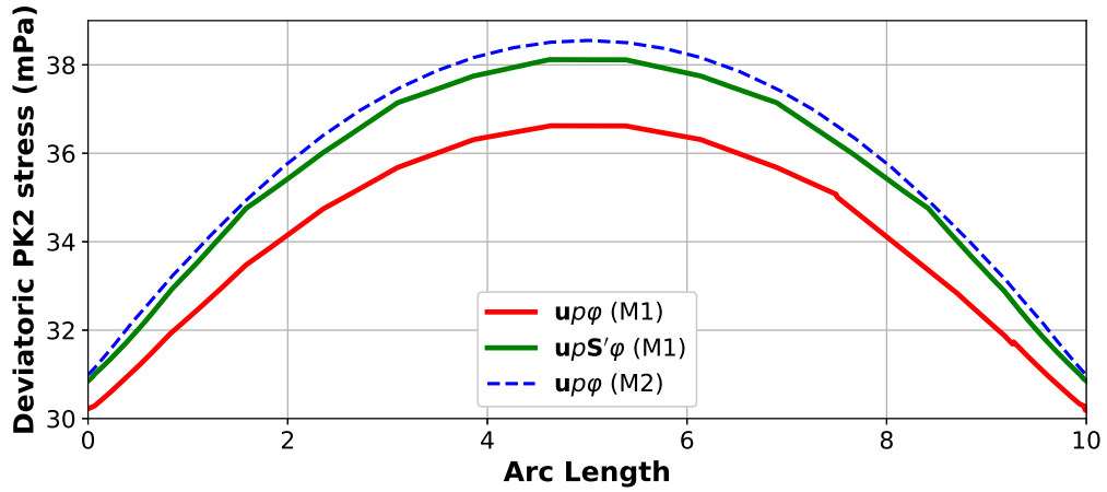
(B) Deviatoric PK2 mechanical stress magnitude
