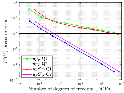
(C) Pressure error upon DOFs
